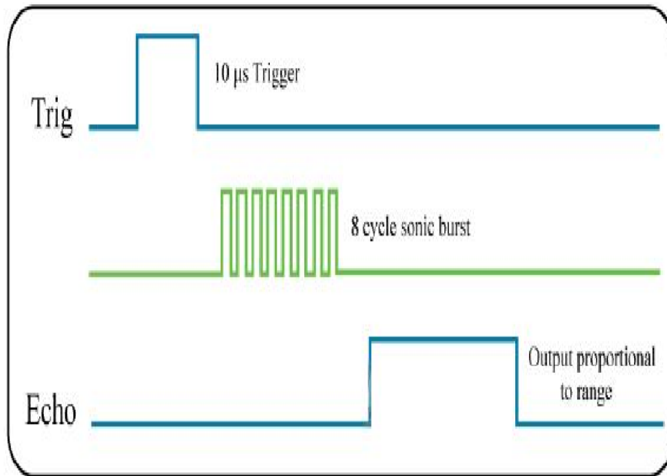
Fig. 4. HC-SR04 timing diagram Source: Etim (2010)
