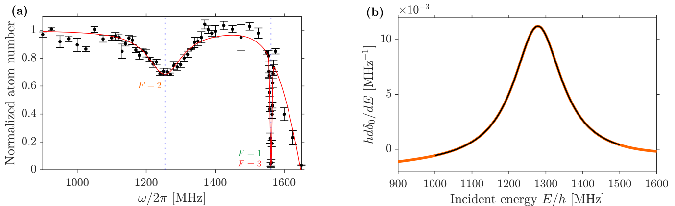
FIG. 2. (a) Photoassociation spectroscopy of \text{Na}_2 molecular states of the \{f = 1, f = 2\} manifold in the presence of a static magnetic field of amplitude B_s = 0.89(1) G. The black circles correspond to the average over three experimental measurements of the remaining atom number after a microwave pulse duration of 80 ms and a microwave field amplitude |B_-| = 5.33 G for \omega \simeq 2\pi \times 1254 MHz. Error bars represent the standard deviation of the different measurements and give an indication of the atom number stability in the experiment. In addition to the atomic hyperfine resonance at 1.77 GHz towards the f = 2 atomic states, visible for frequencies above 1500 MHz, we observe two molecular resonances: a broad resonance at low frequency and a thin resonance closer to the atomic resonance. The broad resonance, fitted with a Lorentzian function, is centered at 1254.1(36) MHz and can be attributed to the F = 2 molecular spin states. Its large width of 172(22) MHz at half maximum is due to predissociation (see text). The thin resonance at 1561.9 MHz corresponds to the F = 1, 3 molecular spin states. (b) Numerical characterization of the energy width of F = 2 molecular states of the \{f = 1, f = 2\} manifold. The orange line corresponds to the energy derivative of the s -wave scattering phase shift \delta_0 as a function of the incident energy E , assuming a single open channel, namely |\{1, 1\}; 2, m_F\rangle . The black line is a Lorentzian function fit supplemented with a linear background representing potential scattering. This leads to a peak energy of E = h \times 1278 MHz, slightly detuned compared to the experimental observations and a width of \gamma = 2\pi \times 160 MHz in excellent agreement with the experimental data.
