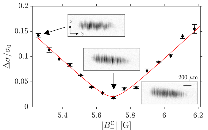
FIG. 8. Ratio of the standard deviation \Delta\sigma with the mean transverse width of the cloud \sigma_0 for different values of the amplitude of |B_-^c| and for fixed |B_-| = 5.53(8) G. This quantity characterizes the amplitude of the cloud excitation when the AC Zeeman shift is not perfectly compensated (see text for details). The error bars represent the standard deviation of two measurements. The red line is a guide to the eye. The top left inset shows an absorption imaging picture of the cloud after 10 ms time of flight. The snake shape of the cloud is due to the excitation of the transverse dipole mode of the BEC and to the fact that the transverse oscillating frequency varies by about 10% along the x -direction. The middle inset shows an absorption imaging picture of the cloud when the AC Zeeman effect is optimally compensated at |B_-^c| = 5.70 G. We attribute the slight difference between |B_-^c| and |B_-| to systematic errors in the microwave field calibration (see text). The bottom right inset shows an absorption imaging picture of the cloud when |B_-^c| = |B_-| = 0 G.
