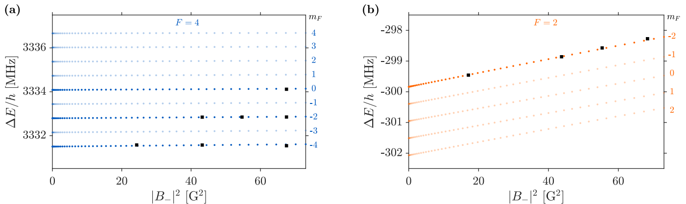
FIG. 5. Two-photon photoassociation spectroscopy for different values of the microwave field amplitude |B_-| and with B_s = 0.92(1) G. Black squares correspond to experimental measurements based on a Lorentzian fit of each resonance (see Table IV of Appendix D). The strong AC Zeeman shift on the atomic transition is compensated relying on a second microwave field as explained in Appendix C. (a) F = 4 molecular states of the \{f = 2, f = 2\} manifold. The blue points correspond to numerical calculations. An offset of -2.99 MHz has been added to the calculated values. (b) F = 2 molecular states of the \{1, 1\} manifold. The orange points correspond to numerical calculations. An offset of -6.13 MHz has been added to the calculated values.
