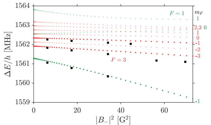
FIG. 6. Photoassociation spectroscopy of the F = 1, 3 molecular states of the \{f = 1, f = 2\} manifold for different values of the microwave field amplitude |B_-| . The static magnetic field is equal to B_s = 0.90(1) G. Black squares correspond to experimental measurements based on a Lorentzian fit of each resonance (see Table V of Appendix D). The colored points correspond to numerical calculations. The strong AC Zeeman shift on the atomic transition is compensated relying on a second microwave field as explained in Appendix C.
