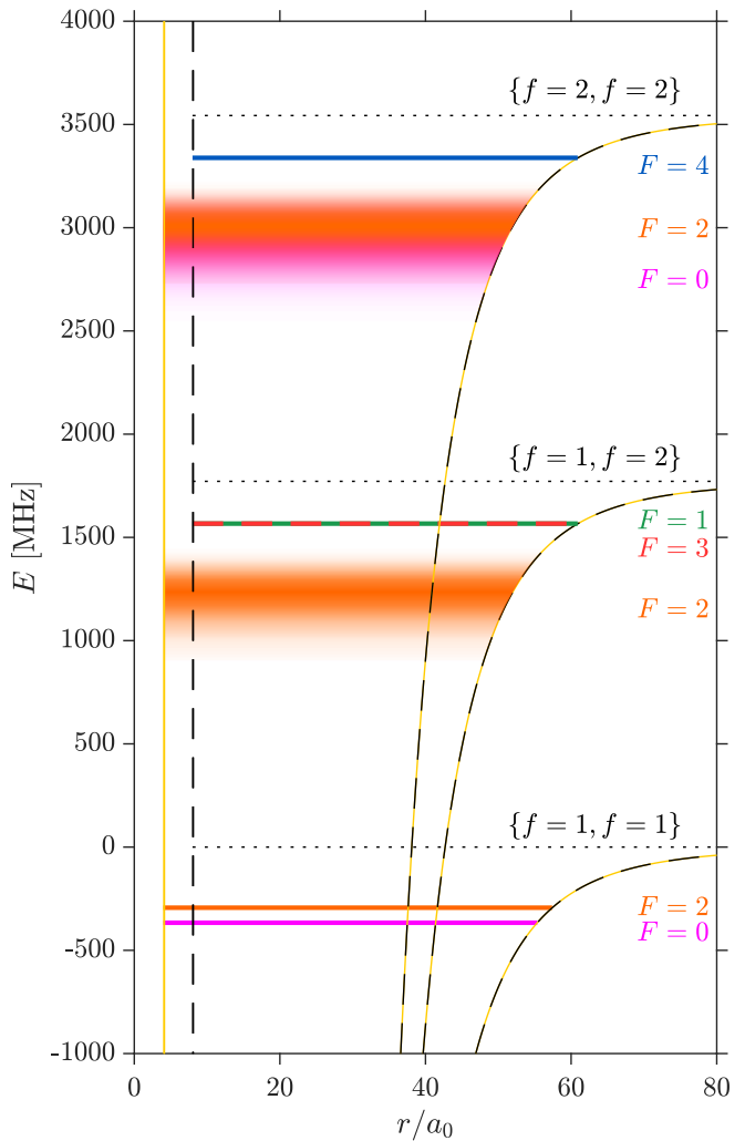
FIG. 1. \text{Na}_2 least-bound states energies (colored lines). Hyperfine interaction distributes these levels between three different manifolds whose dissociation limit is indicated by a black dotted line. The black dashed and yellow solid lines show the triplet interaction potential V_T(r) and singlet interaction potential V_S(r) respectively. F = 1, 3, 4 states are pure triplet states. F = 0 and F = 2 spin states are mixed singlet and triplet states. Within the \{f = 1, f = 2\} and \{f = 2, f = 2\} manifolds this leads to predissociation where the F = 0 and F = 2 molecular states can easily leak out to continuum states. The relative distance r is scaled with a_0 , the Bohr radius.
