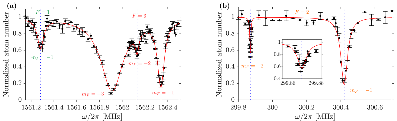
FIG. 3. Photoassociation spectroscopy of \text{Na}_2 molecular states in the presence of a static magnetic field of amplitude B_s = 0.89(1) G. The black disks correspond to the average over three experimental measurements of the remaining atom number after a microwave pulse duration of 30 ms. Error bars represent the standard deviation of the different measurements and give an indication of the atom number stability in the experiment. (a) Photoassociation spectroscopy of the \{f = 1, f = 2\} manifold evidencing the Zeeman structure for a microwave field amplitude |B_-| = 0.66 G. The four resonances correspond to different F, m_F states given in the figure whose coupling is allowed by selection rules. The red line is a fit to a sum of four Lorentzian functions. (b) Photoassociation spectroscopy of F = 2 molecular states of the \{f = 1, f = 1\} manifold for a microwave field amplitude |B_-| = 1.09 G. The very thin resonance at 299.87 MHz is a \pi -polarization microwave resonance corresponding to m_F = -2 , while the broader resonance at 300.42 MHz can be attributed to m_F = -1 . The red line is a fit to the sum of two Lorentzian functions. The inset is a zoom of the m_F = -2 resonance. Detailed results of the fits for each picture are given in Table II of Appendix D.
