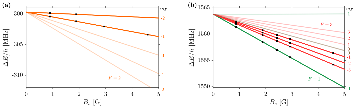
FIG. 4. Photoassociation spectroscopy for different values of the static magnetic field B_s . Black squares correspond to experimental measurements based on a Lorentzian fit of each resonance (see Table III of Appendix D for the microwave pulse parameters used for each point and the detailed fit results). (a) F = 2 molecular states of the \{f = 1, f = 1\} manifold. The orange lines correspond to numerical calculations shifted by -6.13 MHz. (b) F = 1, 3 molecular states of the \{f = 1, f = 2\} manifold. The colored lines correspond to numerical calculations shifted by -2.97 MHz. The brown color of the m_F = 0 states is a symbol for the strong mixing of |\chi_{15}^{1,0}\rangle and |\chi_{15}^{3,0}\rangle by off-diagonal elements of \hat{H}_s , see main text.
