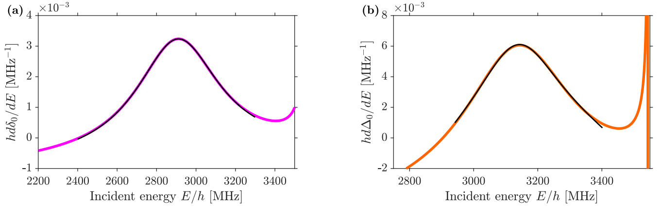
FIG. 7. (a) Numerical characterization of the energy width of the F = 0 molecular state of the \{f = 2, f = 2\} manifold. The purple line corresponds to the energy derivative of the s-wave scattering phase shift \delta_0 as a function of the incident energy E , assuming a single open channel, namely |\{1, 1\}; 0, 0\rangle . The black line is a Lorentzian function fit supplemented with a linear background representing potential scattering. This leads to a peak energy of E = h \times 2908 MHz and a half-width of \gamma/2 = 2\pi \times 258 MHz. (b) Numerical characterization of the energy width of F = 2 molecular states of the \{f = 2, f = 2\} manifold. From the S-matrix defined on the subspace spanned by the two open channels |\{1, 1\}; 2, m_F\rangle and |\{1, 2\}; 2, m_F\rangle , we define the phase \Delta_0 as \det(S) = \exp(2i\Delta_0) . The orange line in the plot corresponds to the energy derivative of \Delta_0 as a function of the incident energy E . The black line is a Lorentzian function fit supplemented with a quadratic background. This leads to a peak energy of E = h \times 3138 MHz and a half-width of \gamma/2 = 2\pi \times 162 MHz.
