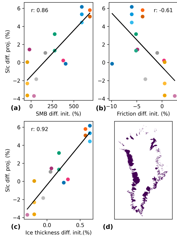
Figure 10. Relative differences in sea-level contribution by 2100 vs. relative differences in filtered and spatially integrated SMB (a), friction coefficient (b), and ice thickness (c) after ice sheet initialization. Black lines in (a–c) denote linear fits. Correlation coefficients as a measure of the goodness of the fit are given within each panel. The color scheme is the same as in Fig. 8. Panel (d) shows the masked area of ERA5-init where surface velocities are larger than 50 \text{ m yr}^{-1} . The mask is used to choose areas over which the SMB, friction coefficient, and ice thickness of each ESM-init are integrated and compared against ERA5-init. Note that the analysis has been proven to be robust to variations in the filter velocity, as similar results have been found with different velocity filters ( 30\text{--}80 \text{ m yr}^{-1} ), as long as the filtered area represents the margin of the ice sheet. For a detailed description, see the main text.
