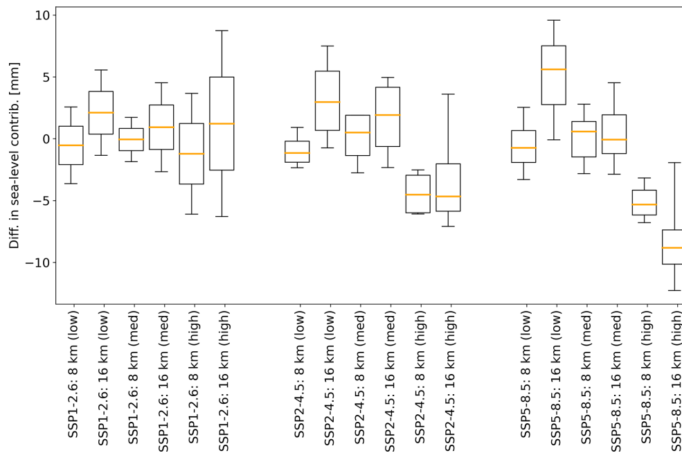
Figure 12. Difference in projected sea-level contribution in 2100 between simulations using different grid sizes. Shown is the difference in simulations run at 8 km (16 km) resolution to simulations run at 4 km resolution. Whiskers show the full range of values; orange lines denote the median.
