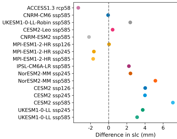
Figure 9. Differences in sea-level contribution (SLC) until 2100 for projections starting from an ESM initial state vs. starting from an ERA5 initial state.
