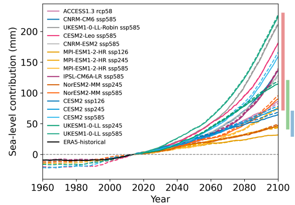
Figure 8. Projected sea-level contributions relative to 2015. Solid lines are projections starting from ERA5-init; dashed lines are the respective ESM-init projections. All simulations were run with medium sensitivity to outlet glacier retreat forcing. Vertical bars denote the range of projected sea-level contribution per scenario: SSP5-8.5 (red), SSP2-4.5 (green), and SSP1-2.6 (blue).
