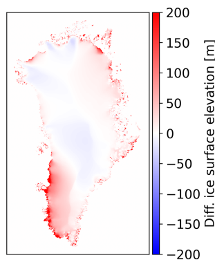
Figure 4. Difference in ice surface elevation compared to ERA5-init for an ice sheet configuration that was spun up with ERA5-SMB and relaxed using NorESM2-MM-SMB.
