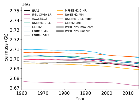
Figure 5. Ice mass over the historical period. All simulations are shown for medium sensitivity to outlet glacier retreat forcing. The grey shadings represent the range of observed mass loss data from Shepherd et al. (2020), with light-grey shading indicating the assumption of maximal error correlation and dark-grey shading indicating uncorrelated errors. The treatment of errors by the Ice Sheet Mass Balance Inter-comparison Exercise (IMBIE) involves two approaches: maximal error correlation assumes that errors across different datasets are fully correlated, leading to a wider uncertainty range (light-grey shading). In contrast, uncorrelated errors assume no correlation between errors in different datasets, resulting in a narrower uncertainty range (dark-grey shading).
