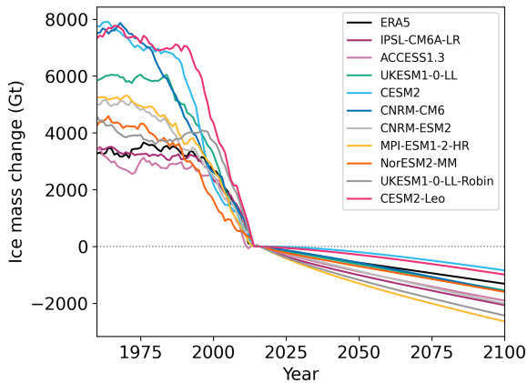
Figure 7. Mass loss (in Gt) of different ice sheet configurations over the historical period and subsequent control projections with forcing set to the mean of the reference period of 1960–1989.
