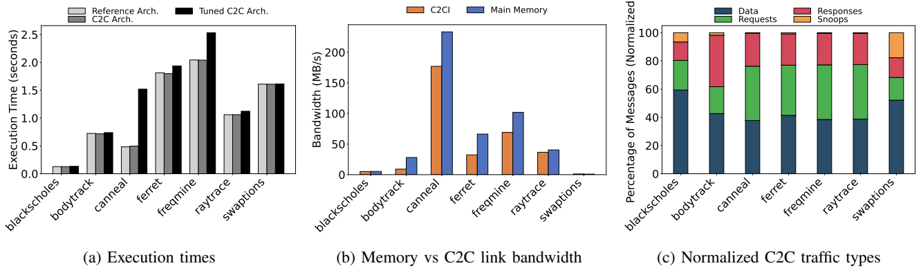
Fig. 7: Comparison of (a) execution times, (b) main memory and C2C link bandwidth, and (c) normalized traffic types for different PARSEC programs across various gem5 architectures: reference single-chip, default chip-to-chip, and calibrated chip-to-chip.
