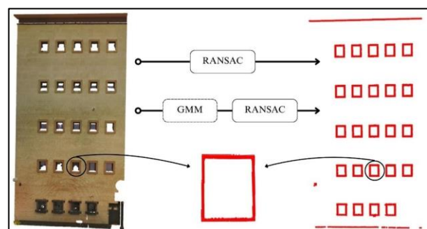
Figure 6. Extraction of a plane by RANSAC (exterior facade)
