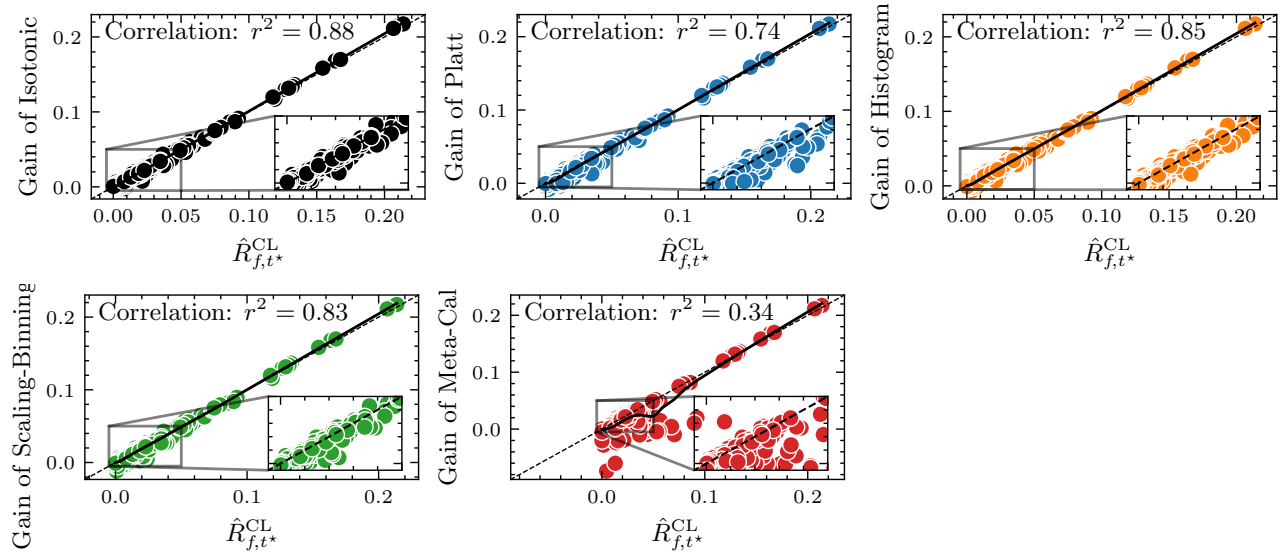
Figure 9: Recalibration gain vs \hat{R}_{f,t^*}^{\text{CL}} . Gain of each recalibration method vs \hat{R}_{f,t^*}^{\text{CL}} .
