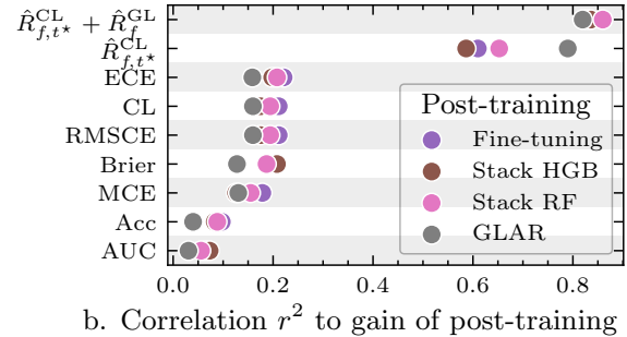
Figure 6: Gain of Post-Training. (a) Gain in utility of fine-tuning versus \hat{R}_{f,t^*} = \hat{R}_{f,t^*}^{\text{CL}} + \hat{R}_f^{\text{GL}} , for each (model, dataset, t^* ). (b) Pearson’s r^2 correlation of the gain in utility of each post-training method with \hat{R}_f^{\text{GL}} , \hat{R}_{f,t}^{\text{CL}} , and other performance metrics.
