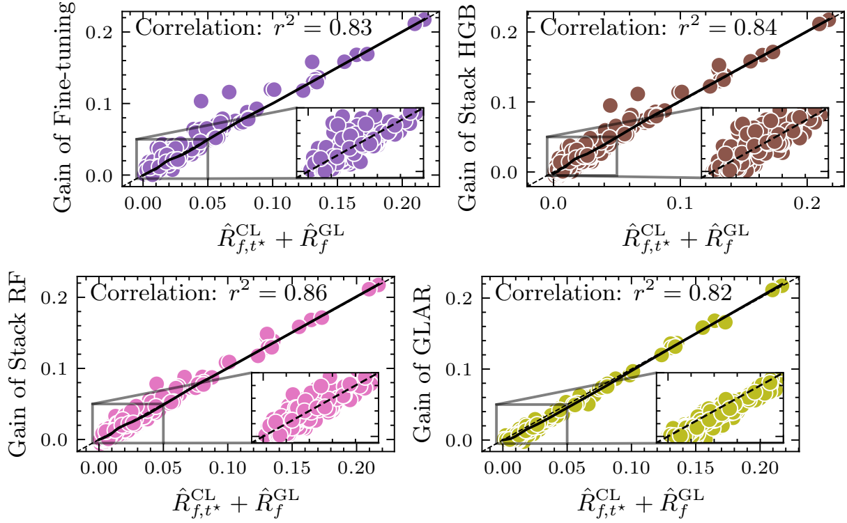
Figure 10: Post-training gain vs \hat{R}_{f,t^*}^{\text{CL}} + \hat{R}_f^{\text{GL}} . Gain of non-recalibration methods vs \hat{R}_{f,t^*}^{\text{CL}} + \hat{R}_f^{\text{GL}} .
