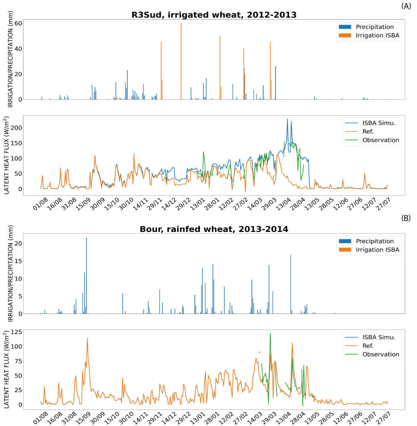
Fig 6. Predictions of latent heat fluxes and irrigation water amounts by the model with and without the irrigation scheme activated for wheat crops, subfigure (A) Predictions for irrigated Wheat (R3_South station) - Period 2012/2013, and (B) Predictions for rainfed Wheat (Bour station) - Period 2013/2014. 'Ref' is for ISBA predictions without irrigation while 'ISBA Simu' stands for ISBA prediction with irrigation.
