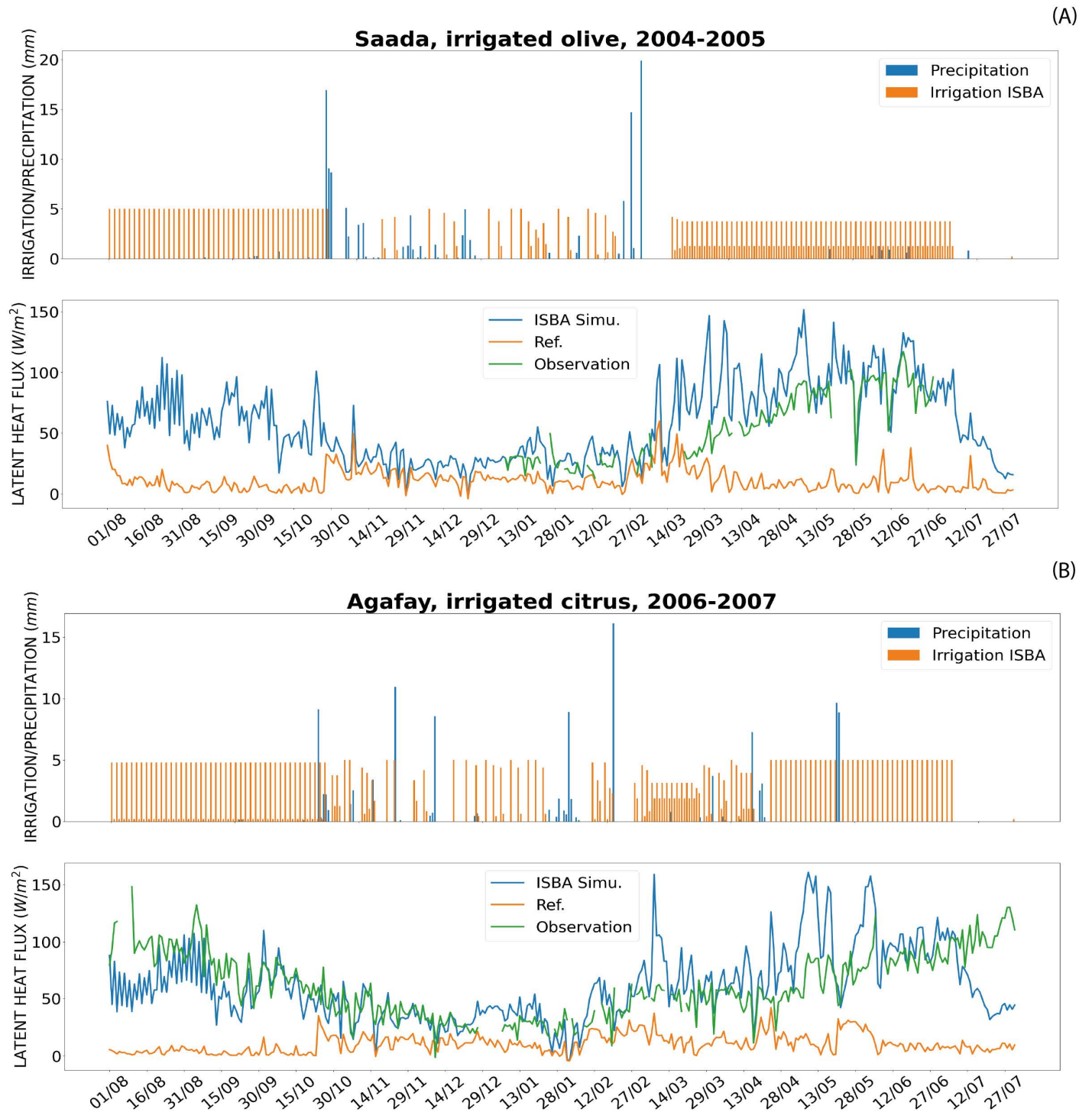
Fig 5. Predictions of latent heat fluxes and irrigation water amounts by the model with and without the irrigation scheme activated for tree crops: subfigure (A) Predictions for olive trees (Saada) - Period 2004/2005, and (B) Predictions for citrus trees (Agafay station) - Period 2006/2007. 'Ref' is for ISBA predictions without irrigation while 'ISBA Simu' stands for ISBA prediction with irrigation.
