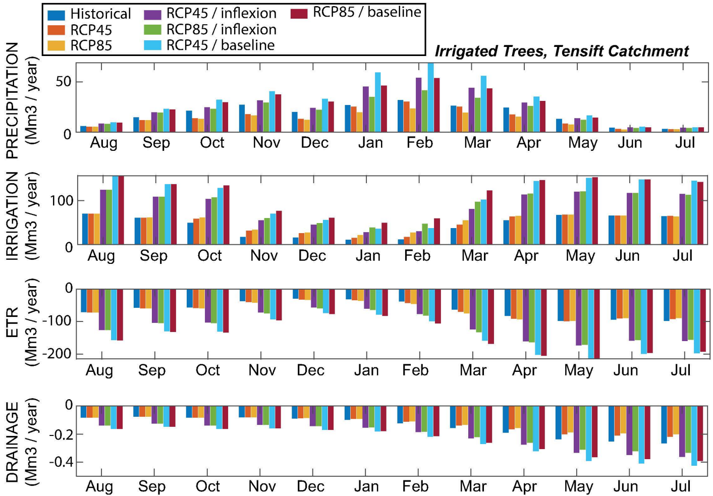
Fig 11. Monthly climatologies of precipitation, irrigation water supply, evapotranspiration and drainage in Mm^3 / year cumulated over all the irrigated tree areas for the historical period and the six scenarios.
