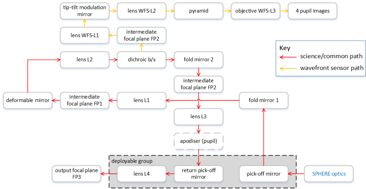
Figure 2. SAXO+ optical functional flow diagram.
