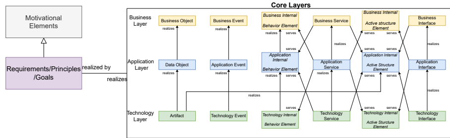
Fig. 6. ArchiMate & TOGAF layers alignment
