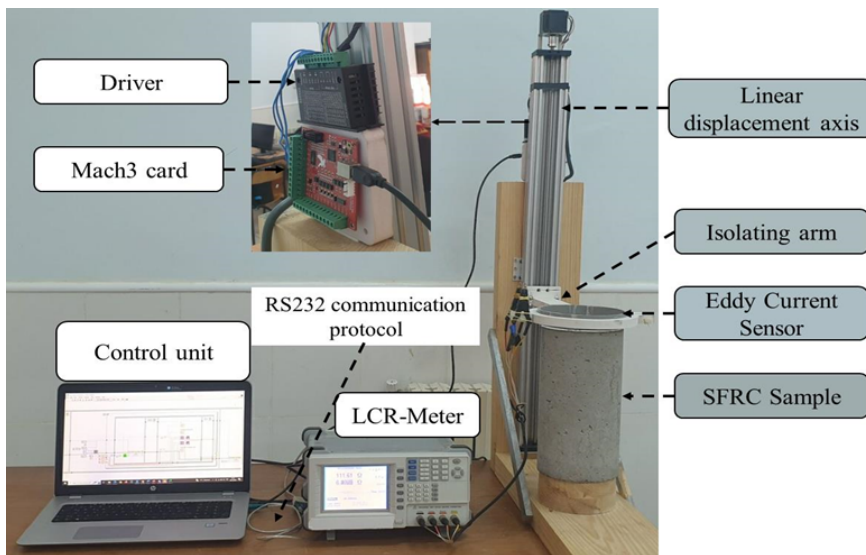
Fig. 1. Measurement system based on Eddy Currents combined with a scanning system.
