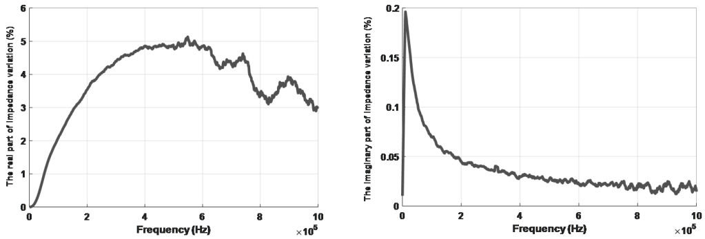
Fig. 6. Relative variation impedance parts according to frequency.
