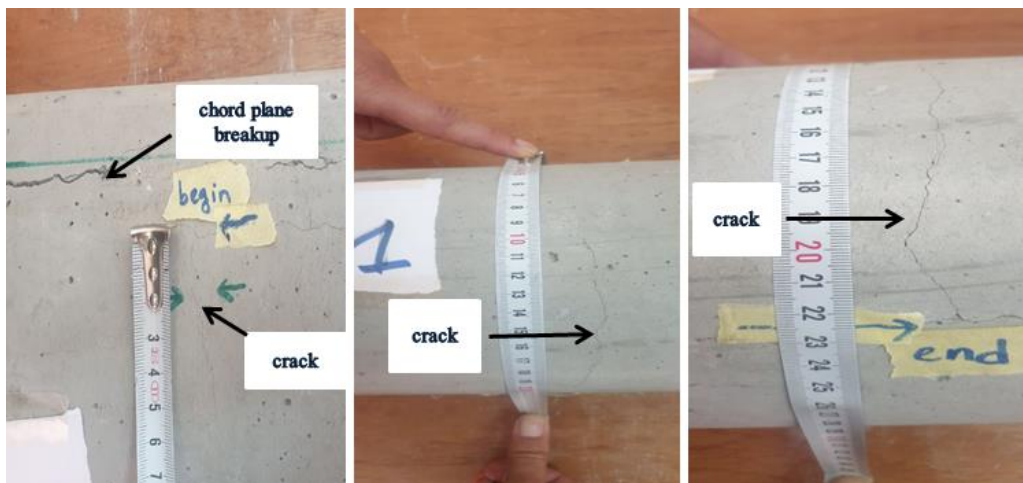
Fig. 13. Course and length of the crack in SFRC Sample A1.
