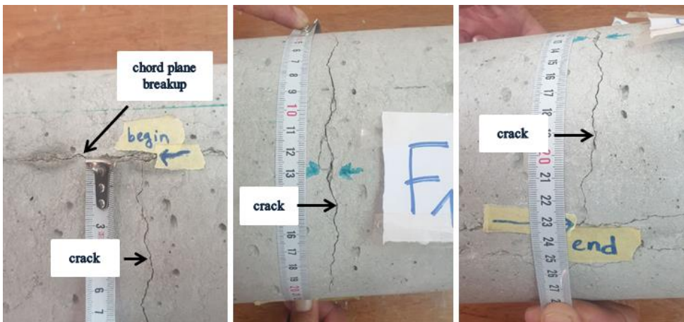
Fig. 16. Course and Length of the Crack in SFRC Sample F1(7).
