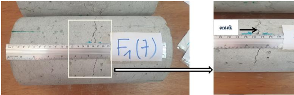
Fig. 15. SFRC Sample F1(7) after undergoing the Brazilian destructive test.
