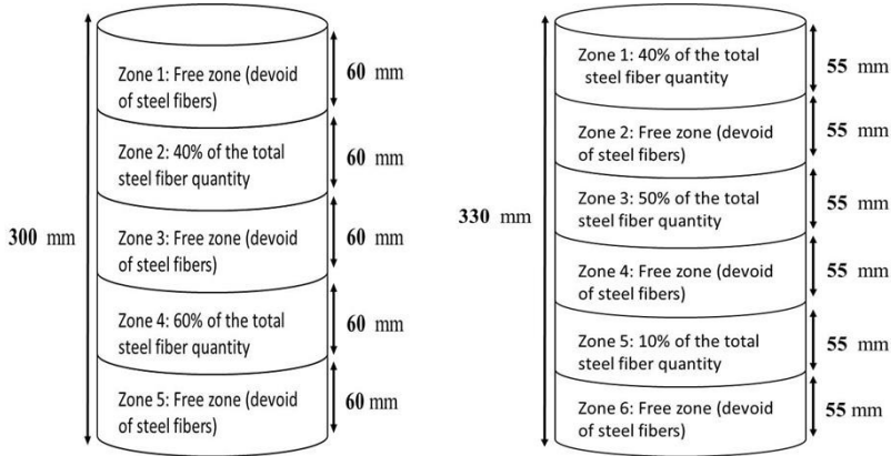
Fig. 7. Zonal distribution of steel Fibers in Samples 1 and 2.
