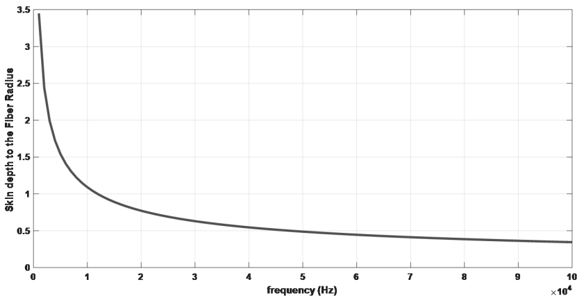
Fig. 5. Ratio of the skin thickness on the fiber radius to frequency.
