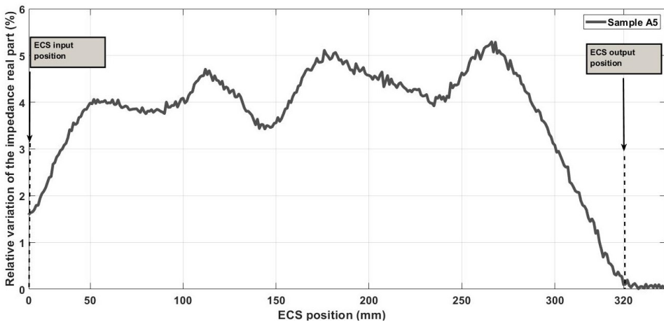
Fig. 21. ECS Impedance Real Part Changes in SFRC Sample A5 according to ECS position.
