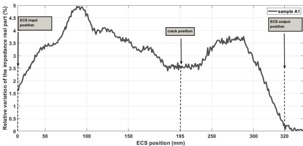
Fig. 14. ECS Impedance Real Part Changes in SFRC Sample A1 according to ECS position.
