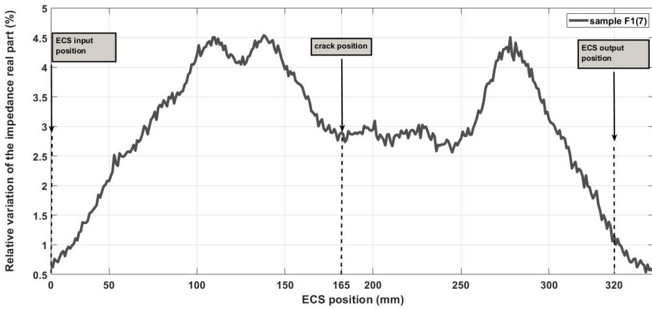
Fig. 17. ECS Impedance Real Part Changes in SFRC Sample F1(7) according to ECS position.
