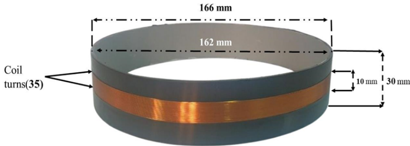
Fig. 2. Eddy current sensor (ECS) dimensions.
