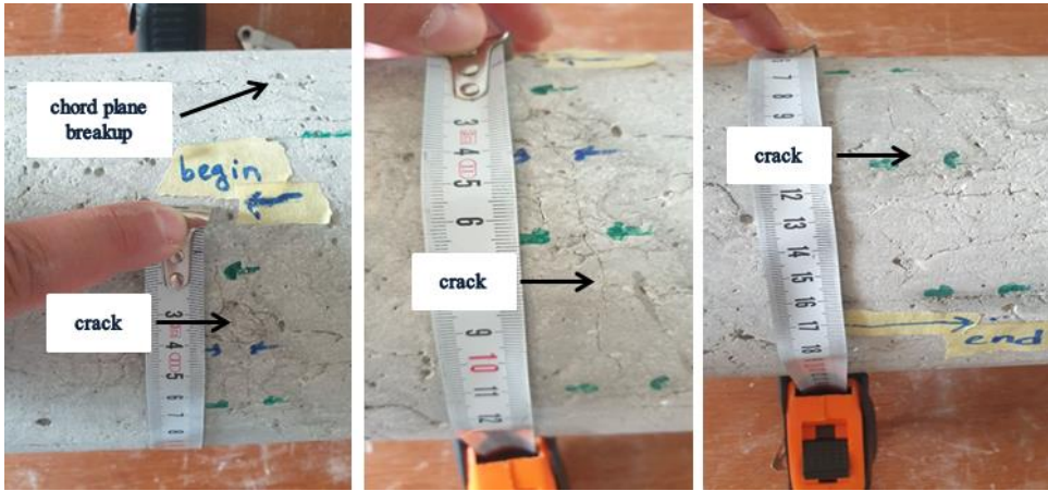
Fig. 19. Course and length of the crack in SFRC Sample F2(4).
