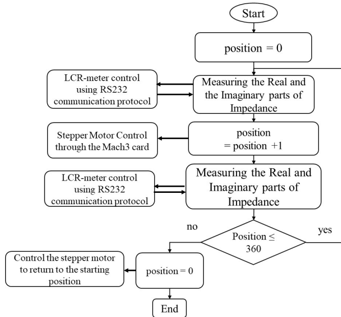
Fig. 3. Operation algorithm of the Eddy Current Non-Destructive scan system.
