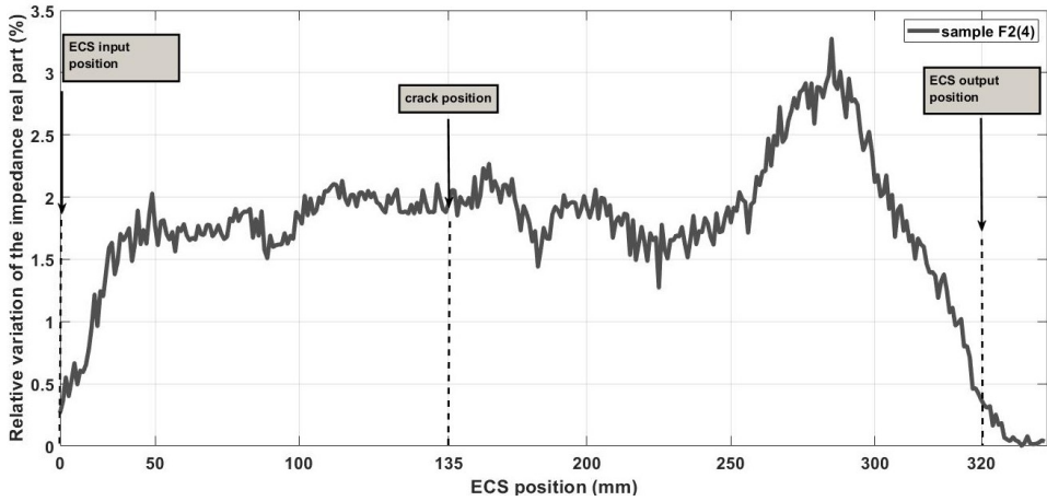
Fig. 20. ECS Impedance Real Part Changes in SFRC Sample F2(4) according to ECS position.
