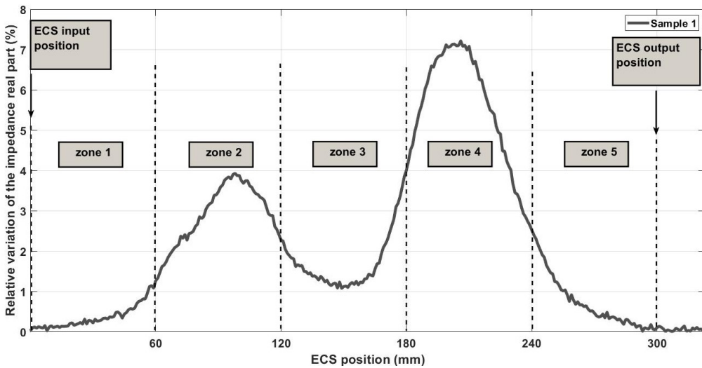
Fig. 8. ECS Impedance Real Part Changes in the SFRC Sample 1 according to the ECS position.
