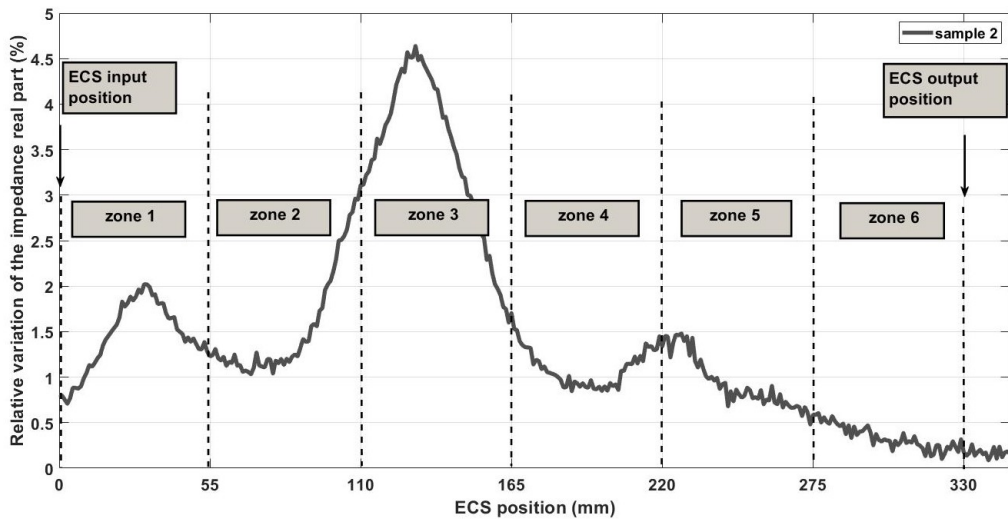
Fig. 9. ECS Impedance Real Part Changes in the SFRC Sample 2 according to ECS position.
