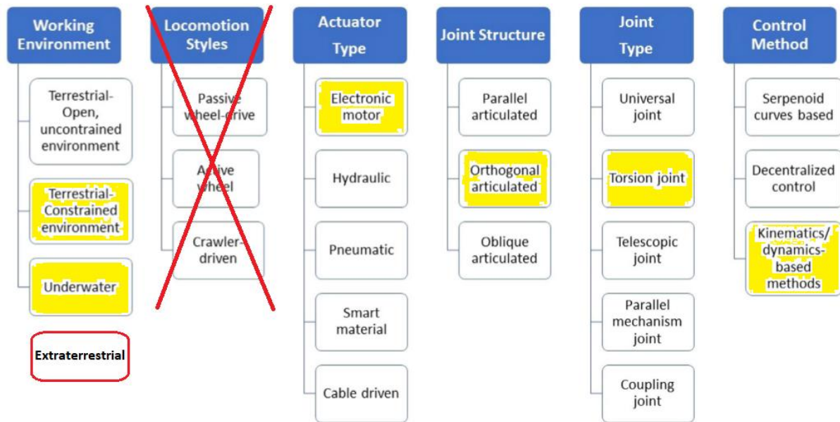
Figure 1. Classification methods of snake robots (figure after [3]). Arm-Z belongs to the class of: constrained, various environments, no locomotion, electric motor, orthogonal, torsion joints, kinematic based control manipulators.
