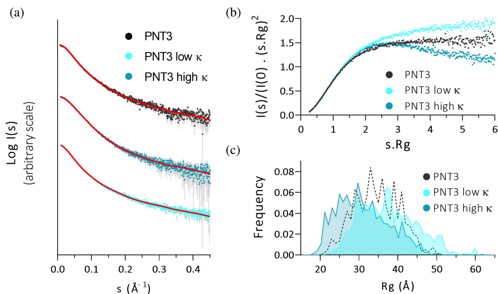
FIGURE 5 Impact of opposite charge distribution on the conformational properties of PNT3. (a) Scattering intensities of wt PNT3, PNT3 low- \kappa , and PNT3 high- \kappa obtained during SEC-SAXS experiments, accompanied by their respective EOM fits (red curves). (b) Corresponding normalized Kratky plots. (c) R_g distribution obtained after EOM deconvolution of the three proteins.
