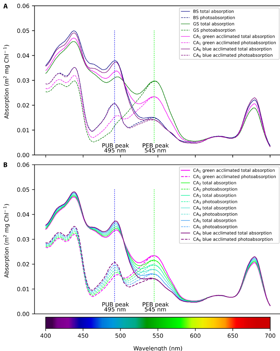
Fig. 2. Total and photosynthetic chlorophyll a -specific absorption spectra of simulated Synechococcus PTs. (A) Total (solid lines) and photosynthetic absorption (dashed lines) spectra of GSs (green lines), BSs (blue lines), and CAs acclimated to blue and green light (indicated by purple and pink lines, respectively). (B) Total (solid) and photosynthetic (dashed) absorption spectra of the CA acclimated to blue and green light (purple and pink lines, respectively) and intermediate acclimation states. The blue and green vertical dotted lines depict the absorption peak of PUB (495 nm) and PEB (545 nm), respectively. “Total absorption” refers to the absorption by all pigments, and “photosynthetic absorption” refers to absorption by only pigments used for photosynthesis (see Materials and Methods and the Supplementary Materials for details).
