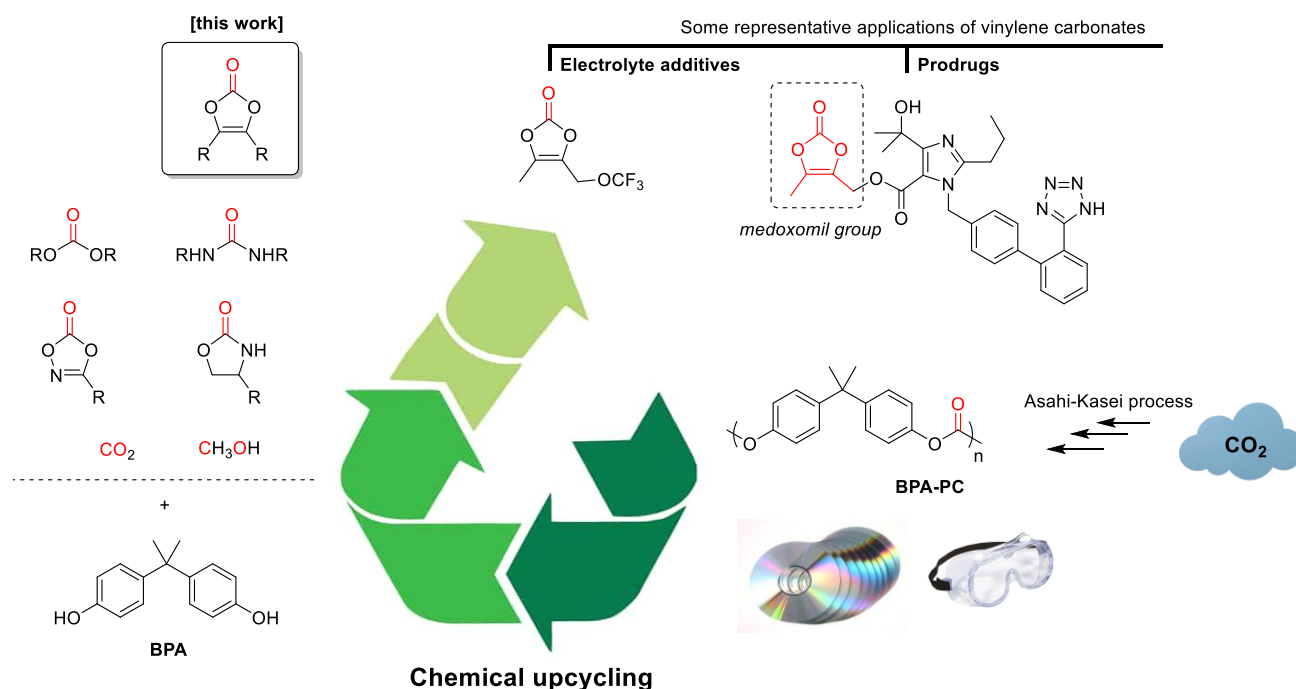
Figure 1. Chemical upcycling of poly(bisphenol A carbonate) to vinylene carbonates and some of their representative applications.
