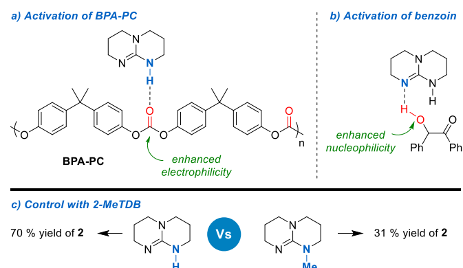
Figure 3. Role of TBD in the depolymerisation process and the formation of vinylene carbonates.
