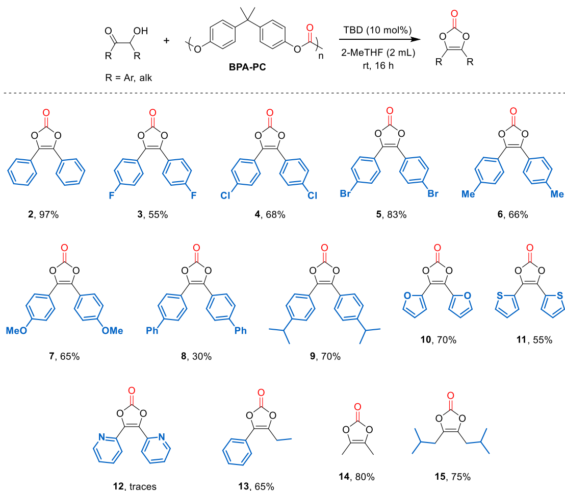
Figure 2. Scope of vinylene carbonates (Isolated yields).
