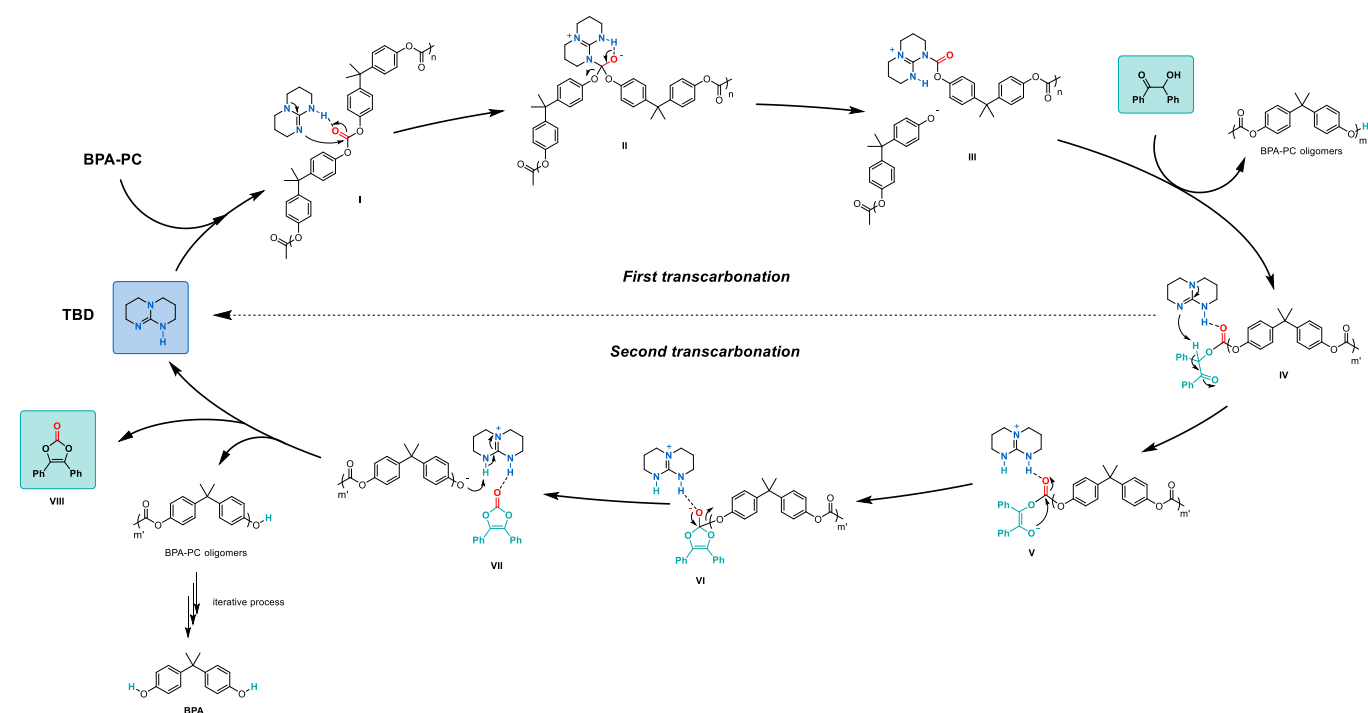
Figure 4. Mechanism proposal for TBD-catalysed depolymerisation of BPA-PC to vinylene carbonates and BPA.
