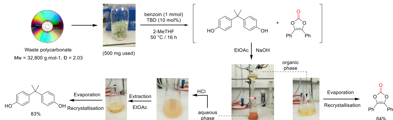
Figure 8. Recovery of vinylene carbonate and BPA from waste polycarbonate contained in compact disk (CD).
