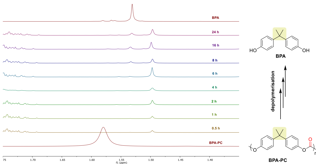
Figure 5. Depolymerisation of BPA-PC followed by ^1\text{H-NMR} (400 MHz, \text{CDCl}_3 , zoom of 1.30-1.75 ppm region corresponding to the gem -dimethyl group). Reaction conditions: benzoin 1 (1 equiv.), BPA-PC (1 equiv.), TBD (10 mol%), 2-MeTHF (2 mL), room temperature. Each aliquot is directly sampled from the reaction mixture and dissolved in \text{CDCl}_3 . Peaks at 1.49 ppm refers to free water found in chloroform.
