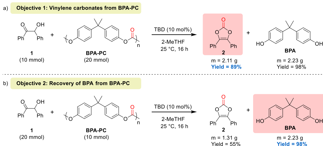
Figure 7. Scale-up reactions for a) the synthesis of vinylene carbonates using BPA-PC as a carbonyl source (objective 1); b) the recovery of BPA from BPA-PC using benzoin as the depolymerisation agent (objective 2). Yields are based on the limiting reagent.
