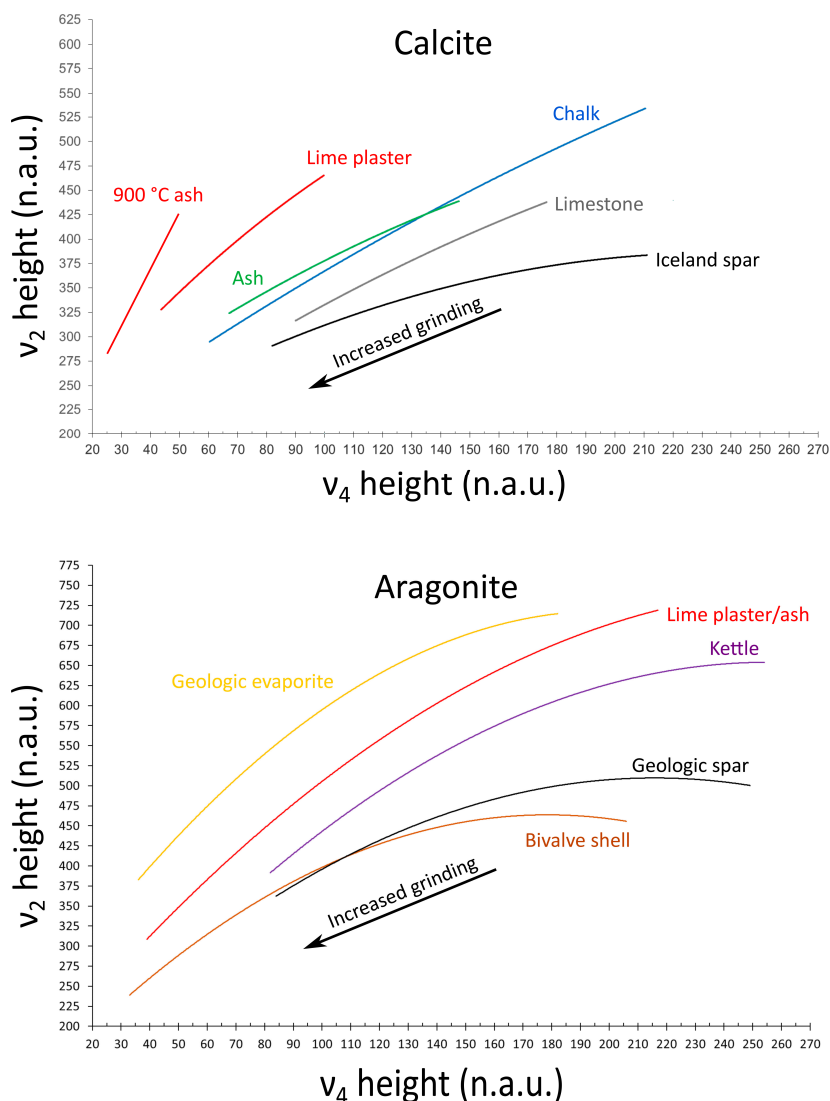
Figure 2. Grinding curves of calcite and aragonite (n.a.u.: normalized absorbance units). Each curve represents a different degree of local structural order and particle size based on calcite and aragonite
