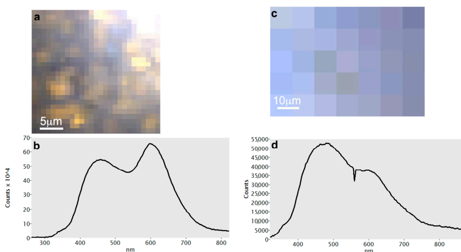
Figure 3. SEM-CL spectra of calcite, modified after Toffolo et al. [87]. (a) Spectrum imaging map of chalk showing emission colors (each pixel corresponds to one measurement); (b) Representative CL spectrum of chalk showing high peak at ~610 nm caused by \text{Mn}^{2+} ; (c) Spectrum imaging map of lime plaster obtained from chalk in (a,b); (d) Representative CL spectrum of lime plaster showing shoulder at ~610 nm caused by displacement of \text{Mn}^{2+} .
