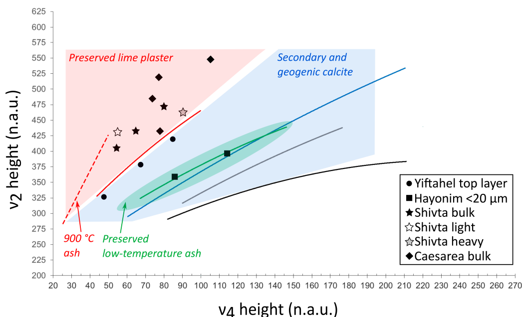
Figure 4. Grinding curves of calcite, showing location of archeological samples (n.a.u.: normalized absorbance units). Trendlines reproduced after Regev et al. [78] with permission from Elsevier; Yiftahel data points modified after Poduska et al. [43]; Hayonim data points modified after Regev et al. [22]; Shivta data points modified after Toffolo et al. [23]; Caesarea data points modified after Asscher et al. [44]. The v_2 and v_4 normalized heights of calcite in archeological samples can be plotted in this chart to determine their degree of preservation.
