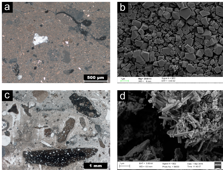
Figure 1. Examples of anthropogenic carbonates. (a) Thin section of Byzantine lime plaster from Shivta (Israel) seen in crossed-polarized light, note the micritic appearance of calcium carbonate crystals; (b) scanning electron microscope (SEM) image of calcite crystals in experimental lime plaster; (c) Thin section of medieval hydraulic mortar from Wilson's Arch (Israel) showing crushed pottery ( cocciopesto ) aggregates; (d) SEM image of acicular aragonite crystals in Iron Age ash from Megiddo (Israel). Detailed data about Shivta and Wilson's Arch in Toffolo et al. [23] and references therein; data about Megiddo in Toffolo et al. [21] and references therein. Figure 1b is reproduced from Toffolo and Boaretto [49] with permission from Elsevier.
