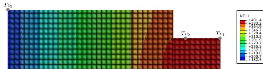
Figure 7. Temperature contourplot in the anvil and the sample at the end of the heating phase ( t = 1100\text{ s} ) for the constant cooling condition.
