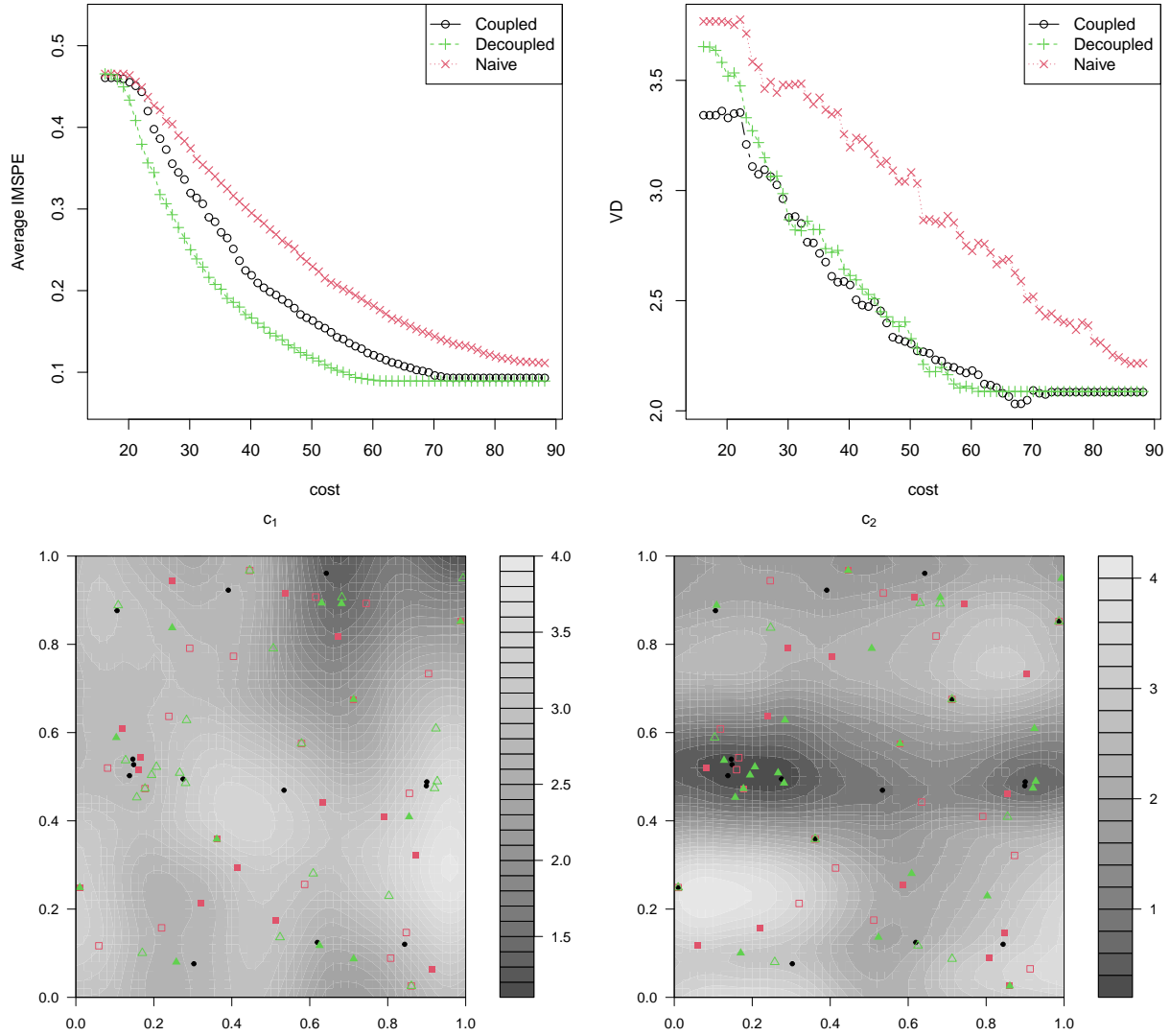
Figure 6: Variable cost for each objective. Top left (resp. right): IMSPE (resp. VD) vs. cost for the various strategies. Bottom: cost surface and evaluated points for each strategy: black dots for coupled, red squares for naïve and green triangles for decoupled. Empty squares and triangles are evaluated on the other objective. naïve doesn't take into account the cost.
