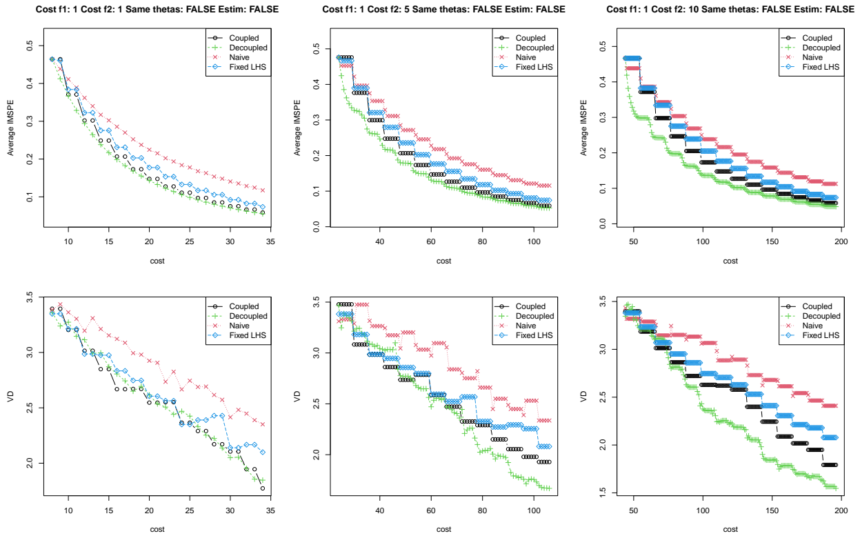
Figure 7: Results of different metrics depending on the cost incurred. In the left column, both objectives have equal cost, in the middle column the cost for f_2 is 5 times as high, and in the right column, the cost for f_2 is 10 times as high. In this figure, lengthscales are equal and assumed known.
