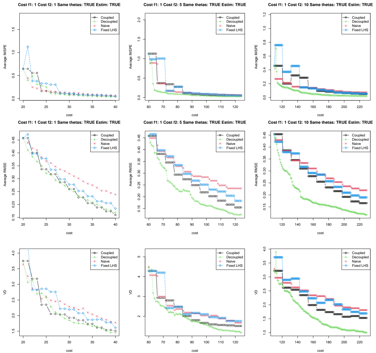
Figure 5: Results of different metrics depending on the cost allocated. In the left column, both objectives have equal cost, in the middle column the cost for f_2 is 5 times as high, and in the right column, the cost for f_2 is 10 times as high. In this figure, lengthscales are equal but unknown (learned and in every iteration).
