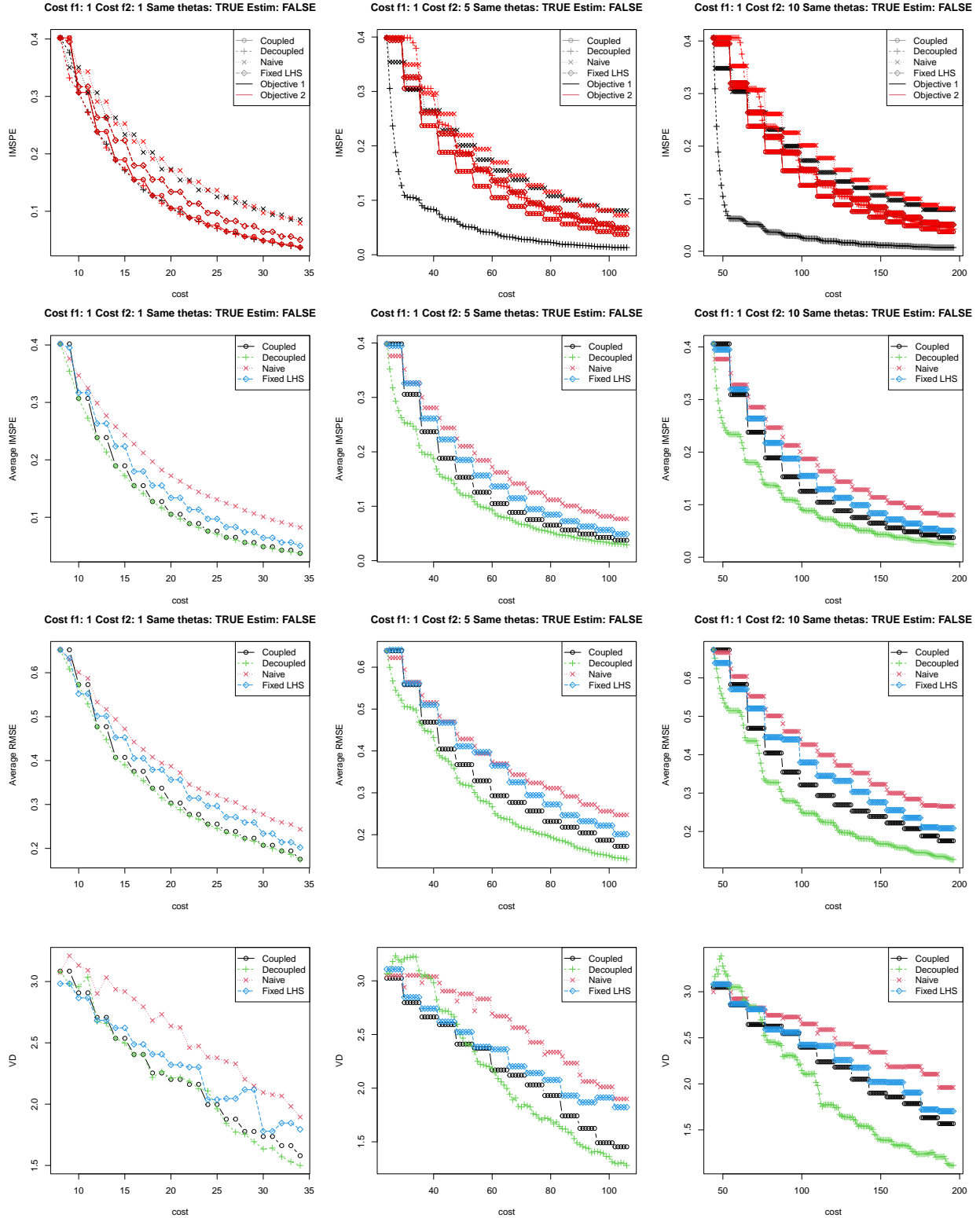
Figure 4: Results of different metrics depending on the cost incurred. In the left column, both objectives have equal cost, in the middle column the cost for f_2 is 5 times as high, and in the right column, the cost for f_2 is 10 times as high. In this figure, lengthscales are equal and assumed known.
