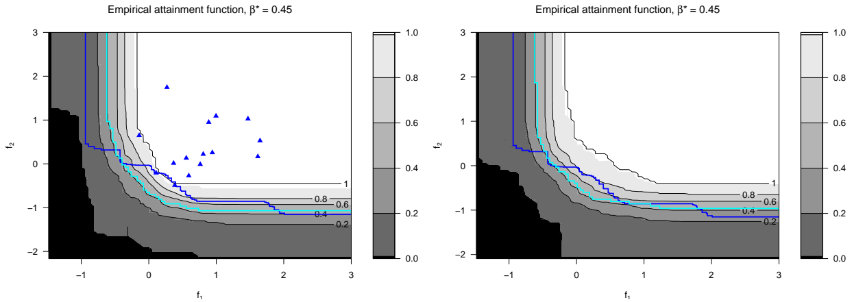
Figure 2: Attainment function representation in the coupled (left) and decoupled (right) cases. The blue triangles mark observations in the coupled case, where both objectives are evaluated. The cyan line represents the estimated Pareto front of the GP while the reference Pareto front is in blue.
