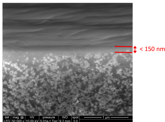
Fig. 13. Low Vacuum SEM image of the unworn sample S1, obtained by cryofracture.
