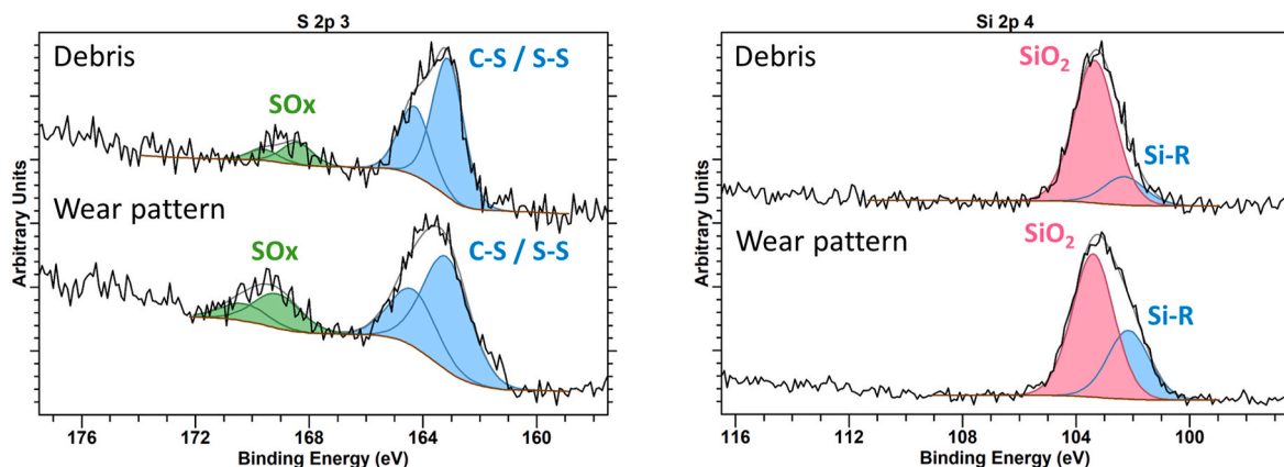
Fig. 16. XPS analyses of the S 2p and Si 2p regions carried out on sample S1. They were obtained on the wear pattern after the whole test process ( F_N = 10 N) and on debris after three wear periods ( F_N = 20 N).
