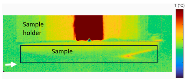
Fig. 11. Image of the thermal measurement of sample S1 during the last wear period. The white arrow indicates the relative displacement of the abrading surface (the sliding direction), and the black rectangle represents the monitored zone used to measure the temperature variations.
