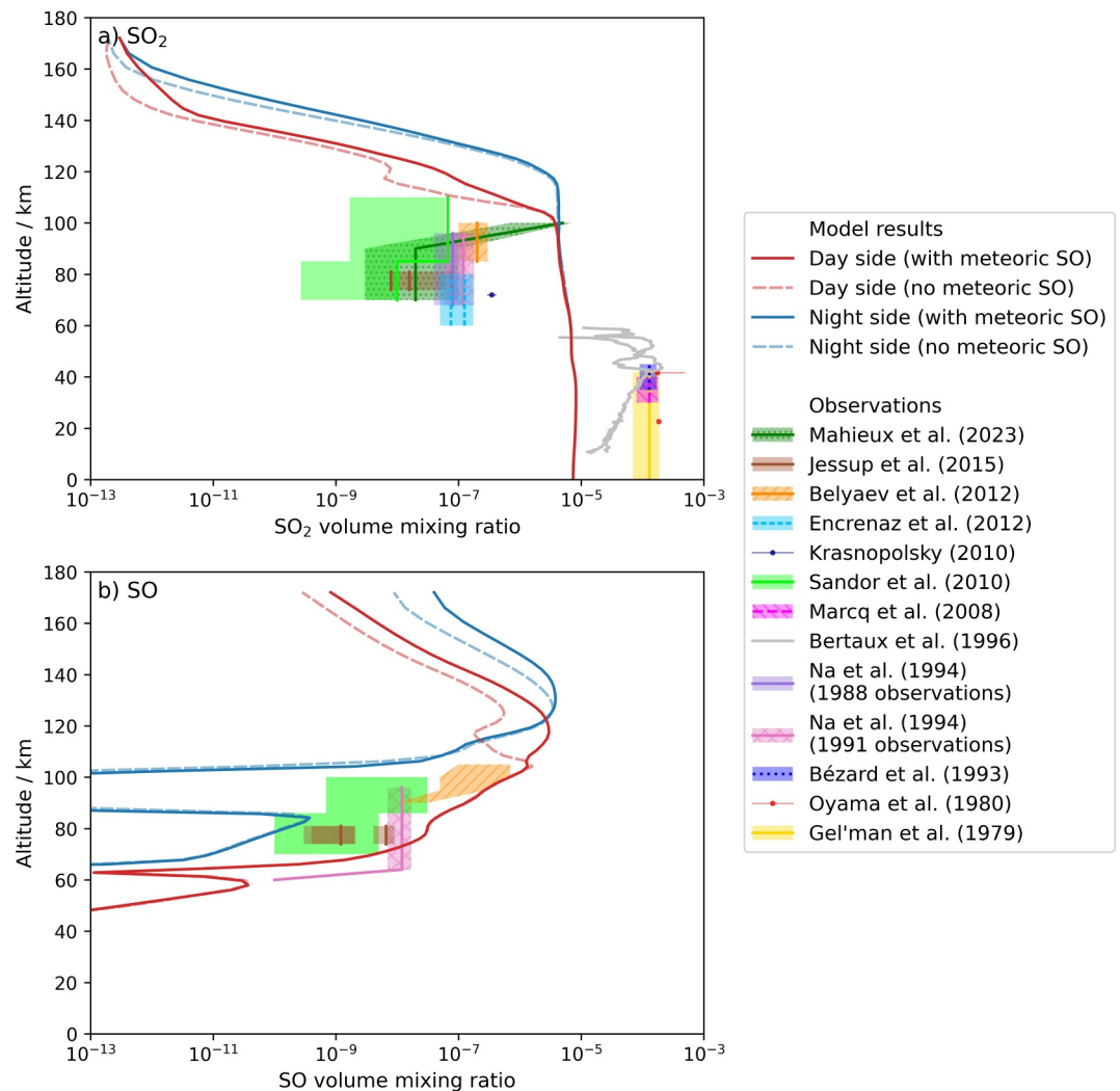
Figure 2. Comparison of (a) \text{SO}_2 and (b) \text{SO} mixing ratio to observations. Model results are averaged from -30^\circ to 30^\circ latitude. Dayside (nightside) is defined as the 140^\circ longitude centered on the subsolar (antisolar) point to prevent capturing terminators. \text{SO} dayside (red) profiles are toward the upper limit of or just above observations. \text{SO}_2 profiles are an order of magnitude too low below the clouds and \sim 3 orders of magnitude too high above the clouds.
