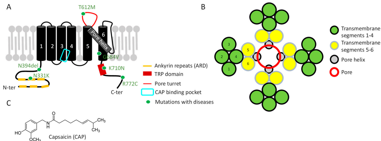
Figure 1. The mammalian TRPV1 channel. (A) Schematic representation of one TRPV1 subunit with the 6 transmembrane segments (S1-S6), a pore turret (red), a pore helix between S5 and S6, an intracellular N-terminal with an ARD, and an intracellular C-terminal with the highly conserved TRP domain. (B) Schematic representation of TRPV1 homotetramer. The S5-S6 pore helix of each subunit is linked to the adjacent subunit to delineate the channel's pore. (C) Structure of CAP, the main agonist of TRPV1. See also [12].
