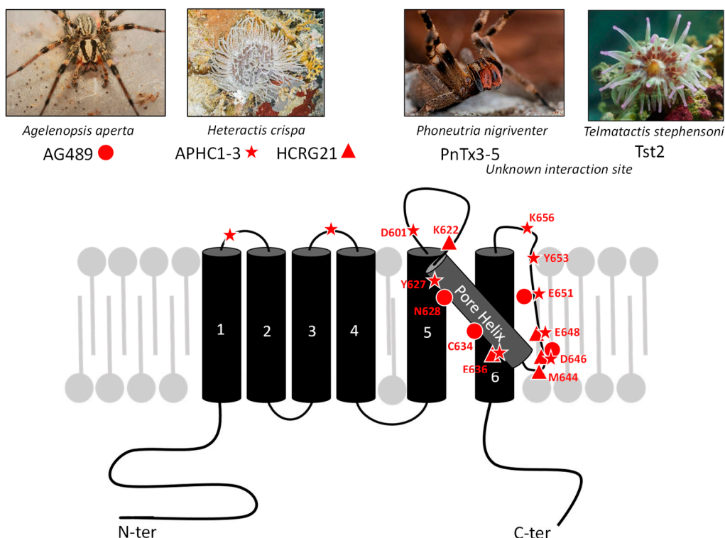
Figure 5. Antagonist toxins and their binding sites on mammalian TRPV1 subunit. Each toxin is associated with its venomous producer. When they are known or suspected, each TRPV1 residue involved in toxin binding is displayed with their respective position in the protein sequence (red numbers). For more details, see [107] for AG489 (●), [108] for PnTx, [109] for APHC (★), and [110] for HCRG21 (▲). All images are from Wikimedia commons.
