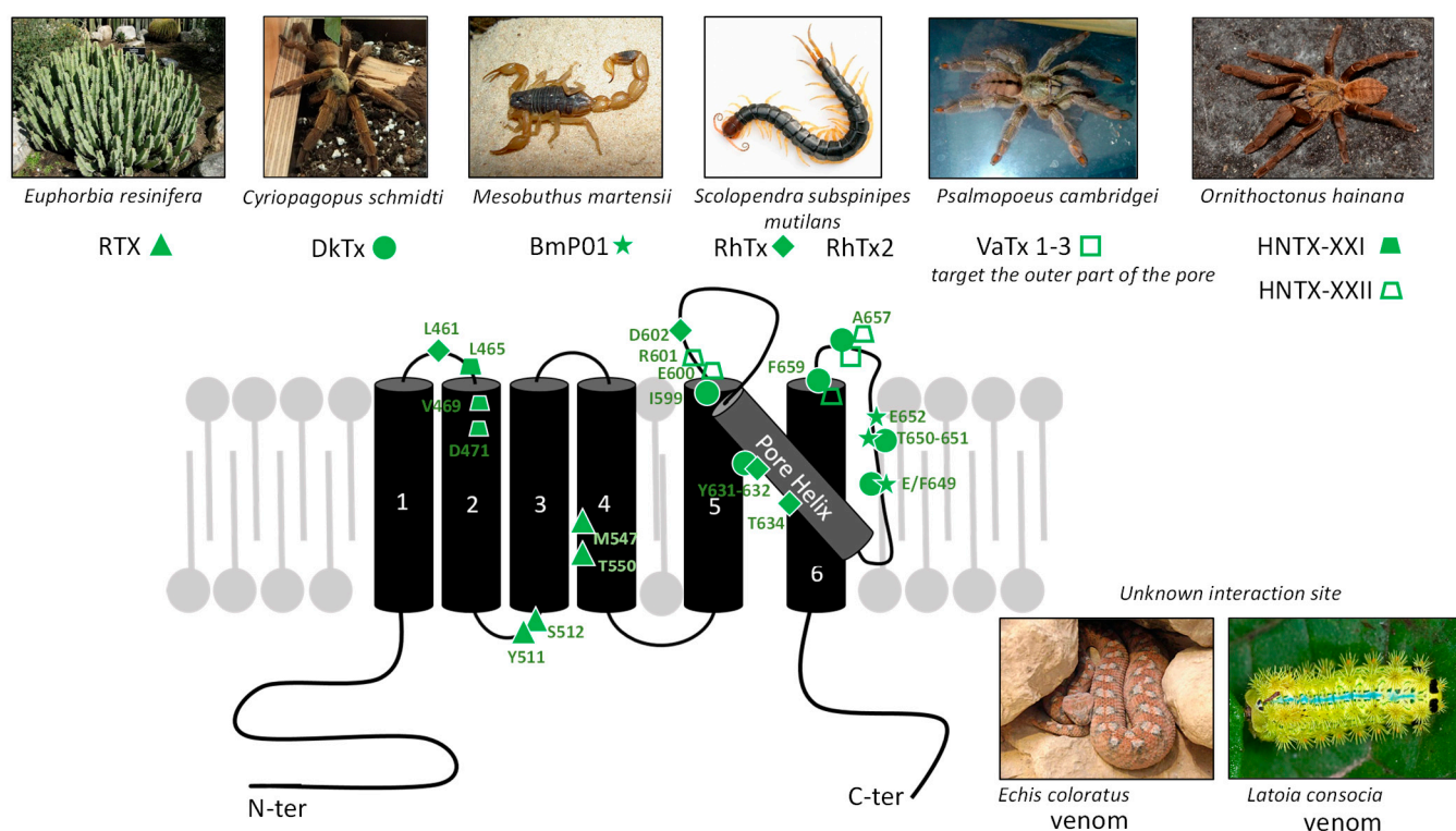
Figure 3. Agonist toxins and their binding sites on a mammalian TRPV1 subunit. Each toxin is associated with its venomous or poisonous producer. When they are known or proposed, each amino-acid residue of TRPV1 involved in toxin bindings site is displayed with its protein position (green numbers). For more details, see [25] for RTX (▲), [87] for VaTx (◻), [92] for DkTx (●), [99] for BmP01 (★), [100,101] for RhTx (◆), and [102] for HNTX-XXI (▲) and HNTX-XXII (◻). Latoia consocia is from ©Daniel Ruyle. All other images are from Wikimedia commons.
