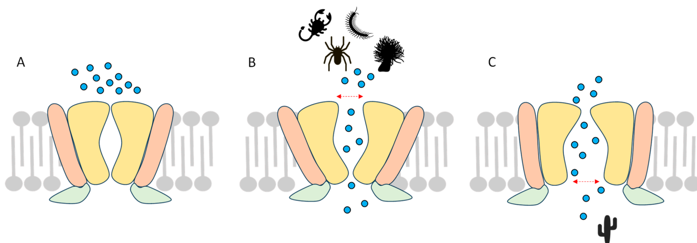
Figure 4. Schematic representation of TRPV1 opening by various agonist toxins. (A) Closed state with cations in the extracellular domain (blue dots). The pore domain is depicted in yellow, S1–S4 transmembrane domains in orange, and the ARD in green. For simplicity, only two subunits are shown. (B) Animal toxins widen the upper pore (red arrow), allowing cations to flow through the channel. (C) Vegetal toxins expand the lower gate through intracellular binding (red arrow).
