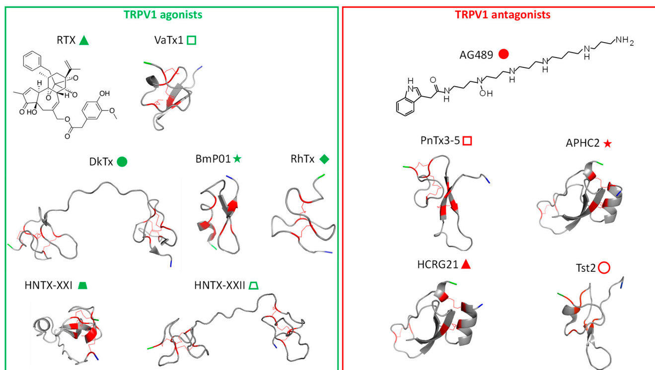
Figure 2. Biochemical and 2D structures of some TRPV1-activating (green symbols) and -inhibiting (red symbols) toxins. HNTX-XXI and HNTX-XXII structures were obtained by homology modeling on the template Hainantoxin-XVIII-7 from Haplopelma hainanum (sequence identity 98.44%; GMQE 0.69) and Tau-Liphistoxin Lth1a_1 from Liphistius thaleban (sequence identity 92.11%; GMQE 0.87), respectively, using Swiss-Model server [78]. PDB ID, AlphaFold ID, and Pubchem structures were used in PyMOL 3.0 software or ACD/ChemSketch freeware 2022.1.0 to design all other molecules. N-term-, C-term-, and disulfide-involved amino acids are labeled in green, blue, and red, respectively. RTX (Wikimedia commons), DkTx (PDB 6CUC), BmP01 (PDB 1WM7), RhTx (PDB 2MWA), VaTx1: Vanillotoxin-1 (AF-P0C244-F1), AG489, PnTx3-5 (AF-P81791-F1), APHC2 (AF-COHJK4-F1), HCRG21 (AF-P0DL86-F1), Tst2 (PDB 8SEM).
