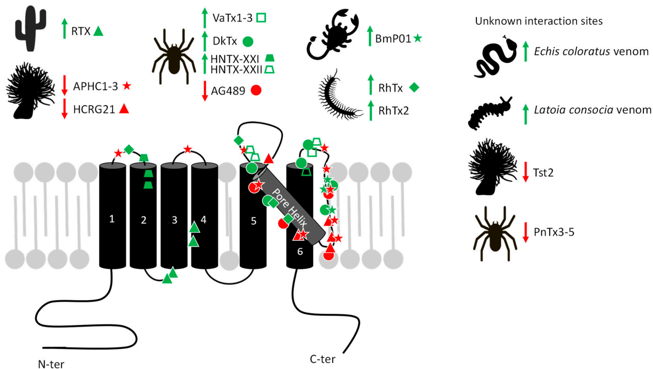
Figure 6. Schematic representation of toxins binding to mammalian TRPV1 subunit, including agonists (green arrows) and antagonists (red arrows) with their ascertained or hypothesized interacting residues. See text for details.
