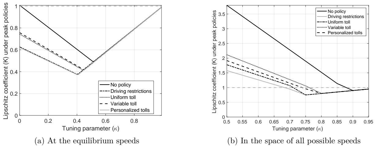
Figure 2: Lipschitz coefficients at the equilibrium speed and for any speed
