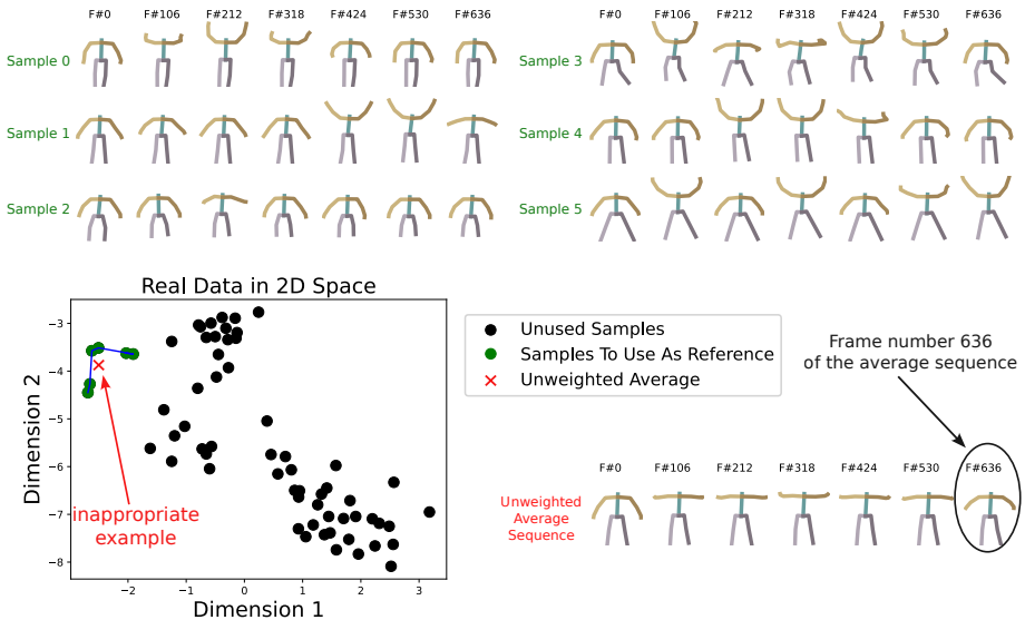
Fig. 2. Averaging six human motion sequences (from Example 0 to Example 5 on the top left/right) assuming a uniformly distributed weight produces an inappropriate distributed example (bottom right skeleton sequence). Following the 2D t-SNE projection of these sequences (bottom left), the placement of the average sequence (bottom left in red) does not belong to the manifold of the original sequences (bottom left in green).
