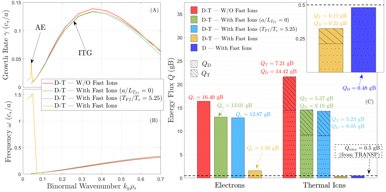
Figure 6: Gyrokinetic analysis of core turbulence reduction in D-T. (A) Growth rate, \gamma , and (B) frequency, \omega , spectrum obtained from linear simulations with the CGYRO code. k_y is the binormal wavenumber normalized to the proton sound gyroradius \rho_s . (C) Energy flux obtained from gyrokinetic simulations performed with the CGYRO code for the discharge #99896 at \rho = 0.31 . The simulations are performed including and excluding the energetic ion component. Values of the ion thermal energy flux deduced from power balance in TRANSP (black horizontal dashed line) are only obtained when the energetic ion component is included in the simulations as a separate species. The total thermal ion energy flux obtained in D-T including energetic ions is compared to the one obtained assuming that all the thermal ions are D while keeping the rest of the parameters fixed. The energy flux in pure D is significantly higher than in D-T (a zoom of those bars is displayed in the inset on the top right). Simulations with a/L_{T_{FI}} = 0 and T_{FI}/T_e = 5.25 are performed to linearly stabilize the low k_y energetic ion mode while keeping the energetic ions in the simulations. Fluxes obtained with stabilized mode and energetic ions cannot reproduce the experimental fluxes.
