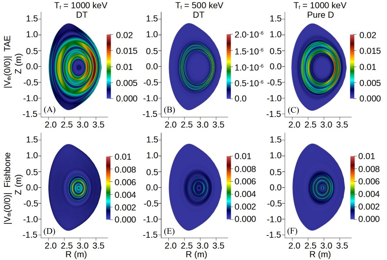
Figure 5: Zonal flow generation by energetic particle instabilities. 2D pattern of n = 0, m = 0 structures of zonal poloidal flows, V_{th}(0,0) , for the TAE and fishbone instabilities. V_{th}(0,0) is defined as V_{th}(0,0) = E_r(0,0) \times B_T with E_r(0,0) the n, m = 0,0 component of the perturbed radial electric field. The dependence of the zonal flow intensity on the perturbation strength is studied by scanning the energetic ion equivalent temperature ( T_f ) using two values, T_f = 1 MeV and T_f = 500 keV in the FAR3D code. Zonal flow generation increases with increasing perturbation intensity for both TAEs (A and B) and fishbones (C and D). The radial extension of zonal flow activity coincides with the extension of the two perturbations. The zonal flow activity in D-T is compared to the one in pure D (E and F) by artificially replacing T by D in FAR3D. The intensity of the zonal flow is lower in D than in D-T.
