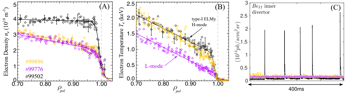
Figure 8: Pedestal characteristics in D-T. Comparison between discharge #99896 and discharge #99502, with P_{NBI} = 12.5 MW, in H-mode with type-I ELMs, and #99776, in L-mode, with P_{NBI} = 5.4 MW and P_{ICRF} = 3.3 MW both obtained at I_p = 2.5 MA, B_T = 3.7 T and q_{95} = 4.5 . (A) Edge n_e . (B) Edge T_e . The profiles are obtained from HRTS averaged in the time window 8.5 s-8.9 s for #99896, 7.3 s-7.6 s for #99502 and 8.6 s-8.9 s for #99776. The evaluation of the error bars in panels (A) and (B) is done by deriving the expected signal levels at a given temperature and by calculating the standard deviation based on the photoelectron statistics, the plasma background light variation and the detector noise. (C) Comparison of the BeII line emission from the inner divertor for the same discharges. The vertical dashed line represents the location of the plasma separatrix.
