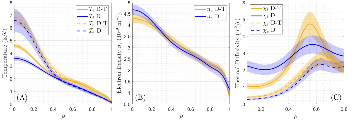
Figure 2: Comparison between the D-T discharge #99896 and the D counterpart #100871. (A) Comparison between T_i and T_e for the D-T discharge #99896 and the D counterpart #100871. T_i is measured by the charge-exchange technique on impurity ions. T_e is obtained by means of LIDAR and high-resolution Thomson scattering (HRTS). An average over 8.5 s-8.7 s is performed. \rho is defined as the square root of the normalized toroidal magnetic flux. Shaded error bars represent standard deviation of the time-averaged signals and the systematic diagnostic uncertainties. (B) Comparison between electron density, n_e , for the D-T discharge #99896 and the D counterpart #100871. n_e is measured with HRTS. Shaded error bars represent standard deviation of the time-averaged signals and the systematic diagnostic uncertainties. (C) Comparison between \chi_i and \chi_e obtained by power balance analysis for the D-T discharge #99896 and the D counterpart #100871. Shaded error bars represent standard deviation.
