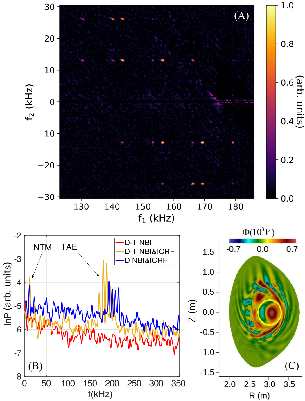
Figure 3: Core plasma fluctuations characteristics. (A) Bicoherence analysis of the perturbations found in discharge #99896. The analysis is performed at t = 7.7 s. (B) Logarithmic power of the density fluctuations as obtained from reflectometry at major radius R \sim 3.36 m, \rho \sim 0.35 and t = 8.4 s, for the D-T discharge #99896 with only NBI heating or with full NBI and ICRF heating and comparison to the pure D discharge #100871. (C) Electrostatic potential, \Phi , fluctuations obtained for the D-T discharge #99896 by the global code FAR3D when considering two species of energetic ions, H and D, accelerated by the ICRF power. The yellow circle represents the q = 1 surface. Inside q = 1 , a n = 1 perturbation is obtained which is identified as a fishbone instability. Outside q = 1 , TAEs are obtained.
