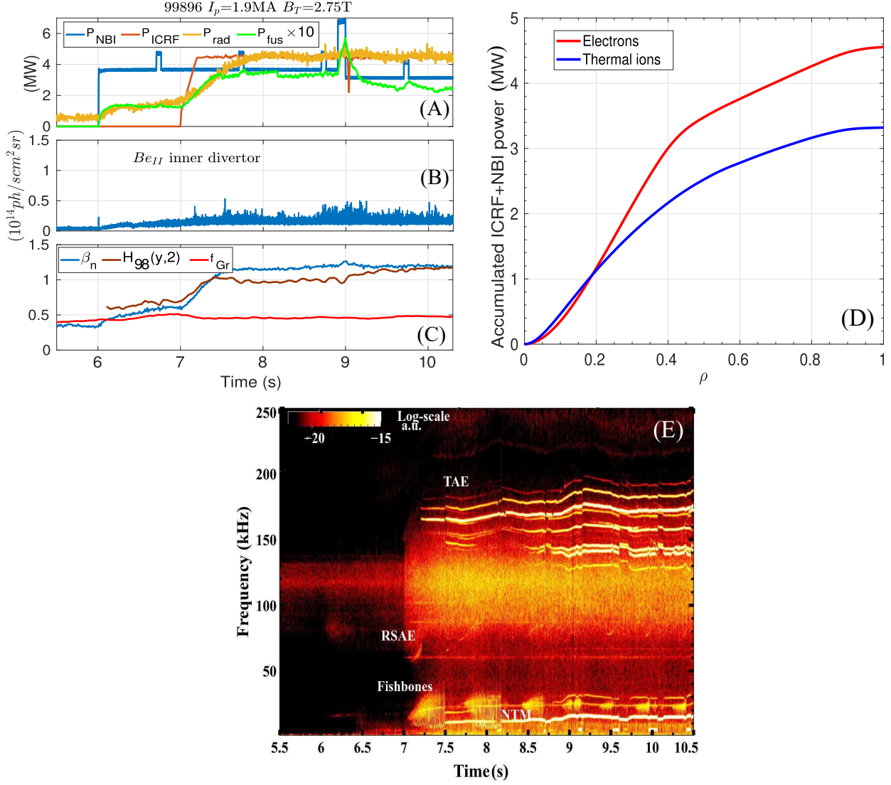
Figure 1: Main characteristics of the D-T discharge #99896. (A) Time evolution of discharge #99896, with toroidal current I_p = 1.9 MA, magnetic field B_T = 2.75 T, and q_{95} = 4.5 , heated mainly with ICRF power, P_{ICRF} = 4.5 MW. The NBI power, P_{NBI} \sim 3.5 MW, was also injected with deuterium beams, before 9 s, and tritium beams, after 9 s. The radiated power, P_{rad} represents 60% of the total input power. The power produced by D-T fusion reactions obtained reaches a maximum of P_{fus} \sim 0.5 MW. (B) Time evolution of edge fluctuations as obtained from the B_{eII} line emission from the inner divertor. (C) Time evolution of \beta_N , defined as \beta_N = \beta a B_T / I_p [%] with \beta the ratio between magnetic and thermal pressure and a the plasma minor radius, H_{98}(y, 2) and f_{Gr} = \bar{n}_e / n_{Gr} the Greenwald fraction with \bar{n}_e the average density and n_{Gr} the Greenwald density defined as n_{Gr} = I_p / \pi a^2 . (D) Accumulated NBI and ICRF radial power deposition for the discharge #99896. (E) Time evolution of magnetic perturbations detected by the Mirnov coils.
