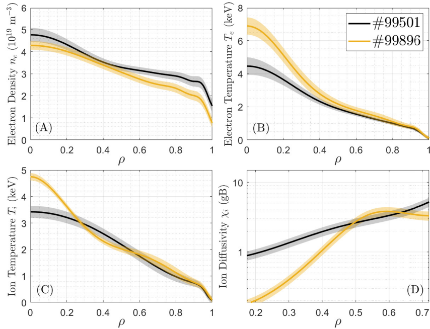
Figure 9: Scenario performance in D-T. Comparison between the discharge #99896, obtained at P_{NBI} = 3.5 MW, P_{ICRF} = 4.5 MW, I_p = 1.9 MA, B_T = 2.75 T and the D-T discharge #99501, obtained at P_{NBI} = 9.5 MW, I_p = 2.5 MA, B_T = 3.7 T. (A) n_e . (B) T_e . (C) T_i . Shaded error bars represent standard deviation of the time-averaged signals and the systematic diagnostic uncertainties in panels (A),(B),(C). (D) \chi_i/\chi_{GB} . \chi_{GB} is the GyroBohm diffusivity defined as \chi_{GB} = T_e^{3/2} m_p^{1/2} / (e^2 B_T^2 a) with m_p the proton mass, e the electron charge and a the plasma minor radius. Shaded error bars represent standard deviation.
