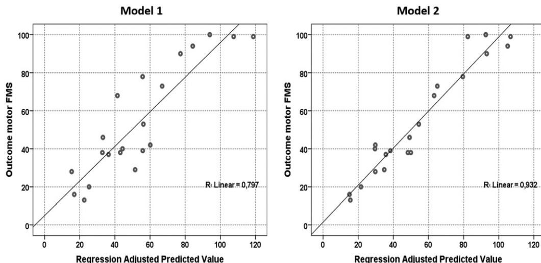
Fig. 6. Plot of predicted and adjusted motor-FMS values for Model 1 ( R^2 = 0.797 ) and Model 2 ( R^2 = 0.932 ).
