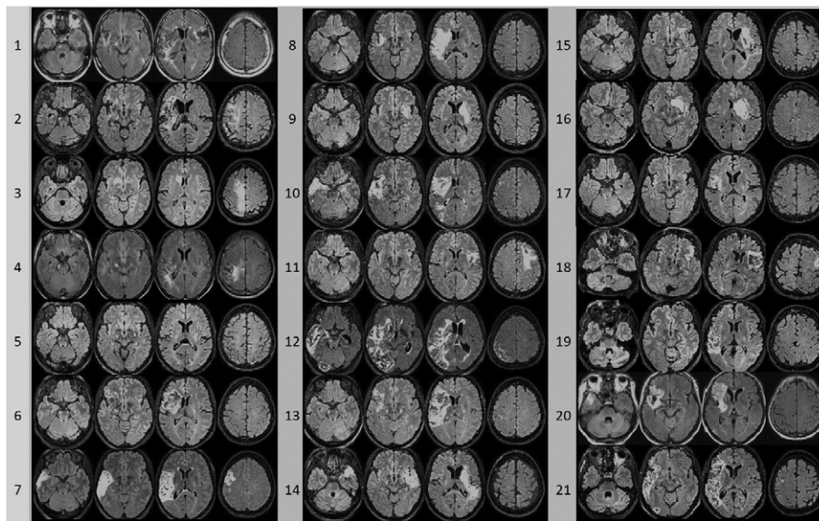
Fig. 2. Four axial slices representative showing stroke lesion extent in 21 patients (FLAIR images).
