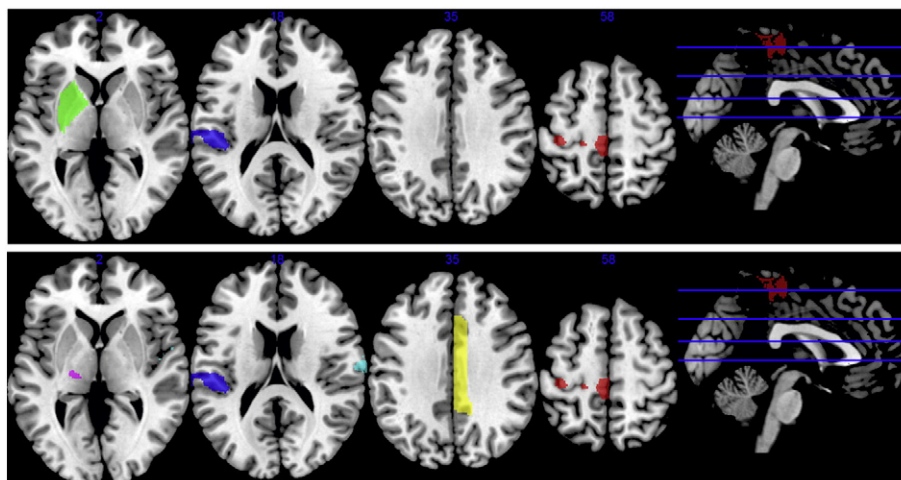
Fig. 5. Upper row: Predictive pattern for Model 1 including baseline motor-FMS including left putamen (green), OP1 (blue) and MI-4a (red). Lower row: Predictive pattern for Model 2 including -fMRI model- showing left OP1 (blue), and thalamus (pink), MI-4a (red), right anterior mid-cingulum (yellow) and OP4 (cyan). The left side indicates the lesioned hemisphere.
