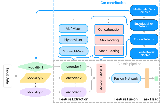
Fig. 1. MixMAS sampling based architecture search pipeline
