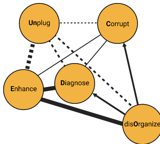
Figure 1. The UnCODE system. The system identifies five classes of qualitatively distinct CogWar goals. The edges represent goal contingencies. Diagnose is centered to illustrate how knowledge is central to reaching CogWar goals. Stapled edges illustrate how Unplug goals eliminate input-output relationships. Narrow edges illustrate how Corrupt goals degrade input-output capacity. Arrows illustrate how disOrganize goals bias input-output activity. Wide edges illustrate how Enhance goals improves input-output capacity.
