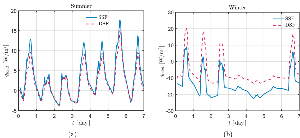
FIGURE 4. Total heat flux density at the glass surface facing the interior ambient for summer (a) and winter period (b).
