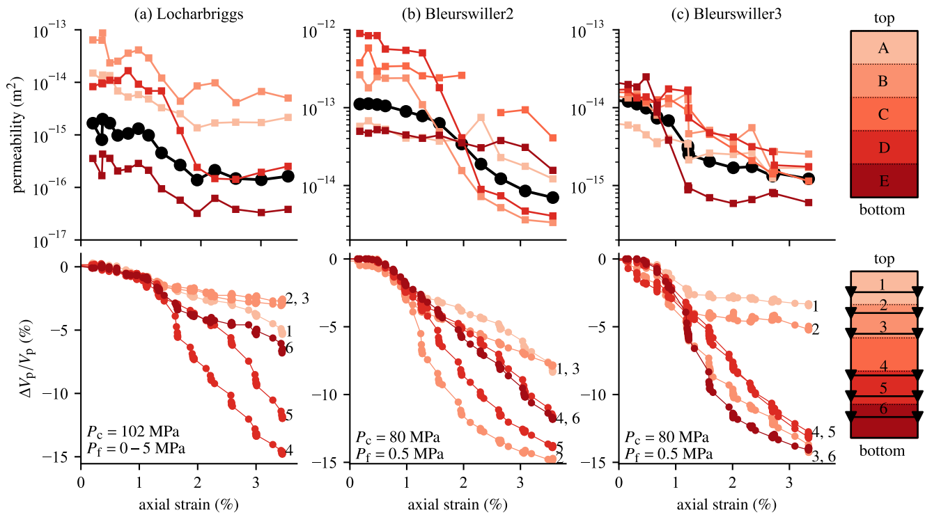
Figure 6. Evolution of permeability and horizontal wave velocities during deformation. (a) Locharbriggs sandstone, (b) Bleurswiller2 sandstone, (c) Bleurswiller3 sandstone. The black curves show the average permeability across the entire sample. All curves are color-coded to match each layer from A (light red) to E (dark red). P wave velocities along horizontal paths are numbered from 1 (top) to 6 (bottom). In Bleurswiller2 sandstone, the permeability at 2.3% in layer C could not be computed because the pore pressure measurements indicated an unphysical, negative pressure gradient in that interval. This error is also likely impacting the permeability inferred in other layers at that strain, with an unexpected increase in layer A. In all rocks, the initial permeability (at zero strain) reported in each plot might differ slightly from that reported in Figure 4 because the measurements were conducted approximately 1 day apart, during which some time-dependent compaction may have occurred.
