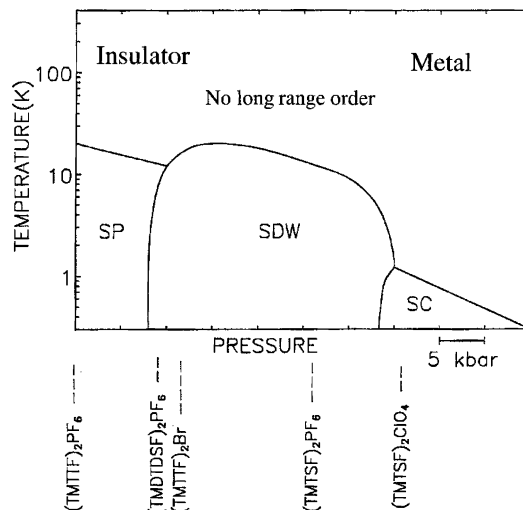
Figure 21. Generic phase diagram for the (\text{TM})_2\text{X} compounds. (Adapted with permission from Science ( http://www.aas.org ), ref 95. Copyright 1991 American Association for the Advancement of Science.)
