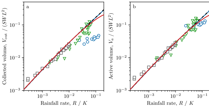
Figure 18: (a) Dimensionless volume of water collected at the aquifer outlet as a function of the dimensionless rainfall rate. (b) Dimensionless active volume of water as a function of the dimensionless rainfall rate. The active volume of water is evaluated from the volume collected at the aquifer outlet, using equation (7.6). Different markers indicate different experimental series (see legend of figure 10). Blue line: infinitely-deep aquifer theory. Red line: weak-rainfall limit of the infinitely-deep aquifer theory, equation (7.8). Dashed black line: numerical computation for an aquifer of aspect ratio a = 0.7 .
