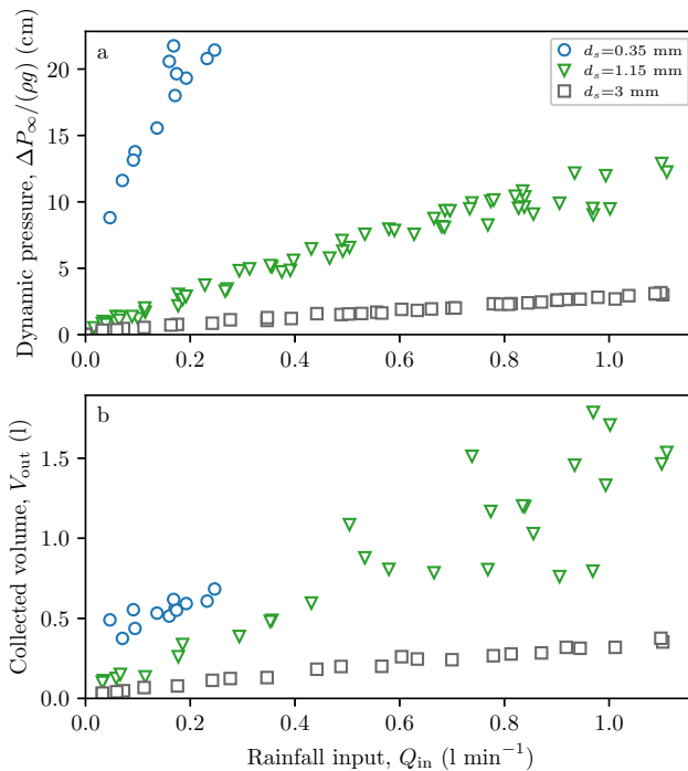
Figure 4: (a) Dynamic pressure (cm of water) and (b) volume of water collected at the aquifer outlet after the rainfall has stopped (l) vs rainfall discharge Q_{in} ( l \text{ min}^{-1} ). Different symbols represent different experimental series (table 1).
