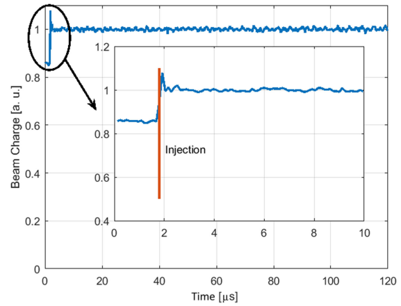
FIG. 17. Beam storage in the ring over 0.12 ms at the rf frequency of 500.38 MHz. An inset provides a close-up view of the first 10 \mu s of the storage process.
