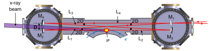
FIG. 28. Schematic drawing of the Fabry-Perot cavity. M_2 and M_3 are the two spherical mirrors and M_1 and M_4 the two planar mirrors. The optical axis (bow-tie shape) is also shown, together with the beam axes incident and reflected by M_1 . Design values of the other geometrical parameters: the incident angle of the optical axis on the cavity mirror surfaces \Theta = 21 mrad, D = 9.5 cm, L_1 = L_3 = 2.2509 m, L_2 = 2.2502 m, and L_4 = 2.2475 m.
