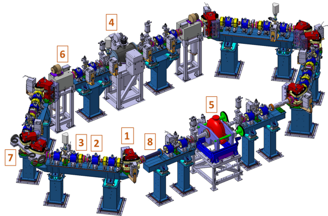
FIG. 14. ThomX storage ring layout. Shown in the figure are 1: 8 dipoles (red), 2: 24 quadrupoles (blue), 3: 12 sextupoles (yellow), 4: septum, 5: rf cavity, 6: 2 kickers (injection/extraction), 7: IP chamber, and 8: feedback transverse stripline.
