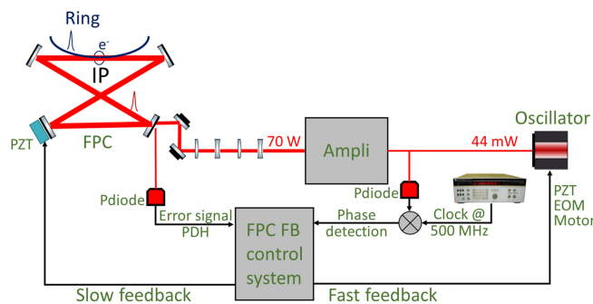
FIG. 33. Simplified scheme of the optical setup and block diagram of the two feedback control loops. “FPC” means fabry-perot cavity, “FB” feedback, “PDH” pound-drever-hall, “PZT” piezoelectric transducer, “EOM” electro-optical modulator, and “Pdiode” photodiode.
