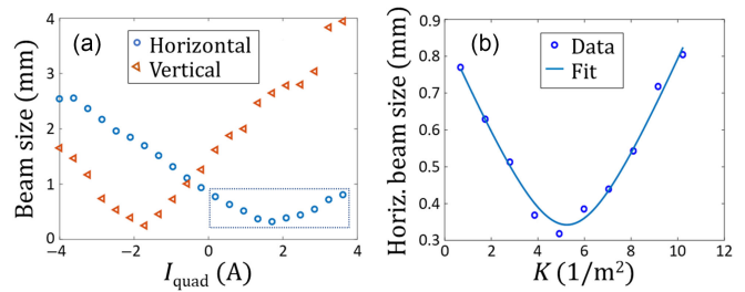
FIG. 10. Example of experimental quad scan at focusing solenoid current of 215 A (a) and scan processing to obtain beam emittance (b), which was found equal to 1.3 \pi mm mrad. The fitted line represents the square root of a parabolic fit of the squared beam size. I_{\text{quad}} is the quadrupole current, and K the quadrupole strength.
