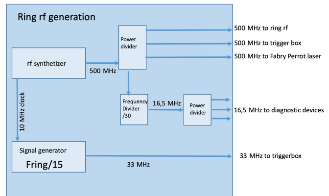
FIG. 36. Block diagram of the ring LLRF distribution scheme.
