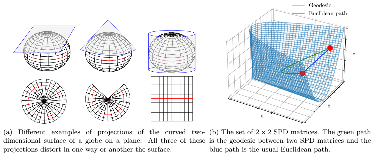
Figure 1: Illustration of the distortion induced by a projection and the set of 2 \times 2 SPD matrices.
