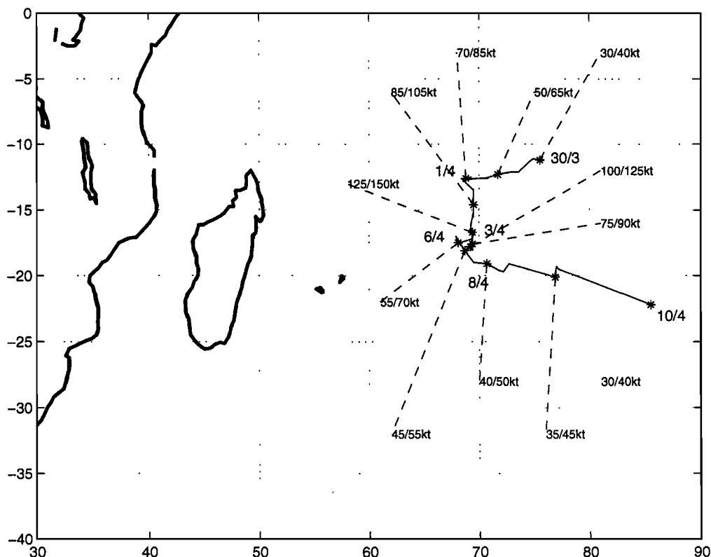
Figure 7. Track of the eye of the cyclone Marlene. Maximum sustained wind and gusts in storm are indicated each day, using knot units (1 kt = 0.51 \text{ m s}^{-1} ).
