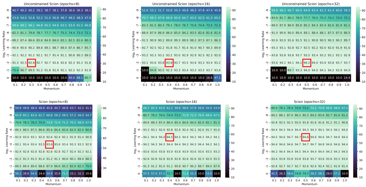
Figure 7. The optimal hyperparameters for (UNCONSTRAINED) SCION on the airbench setting with increasing total number of epochs (indicated in red). SCION outperforms UNCONSTRAINED SCION, which is not surprising since norm control is important in the setting.
