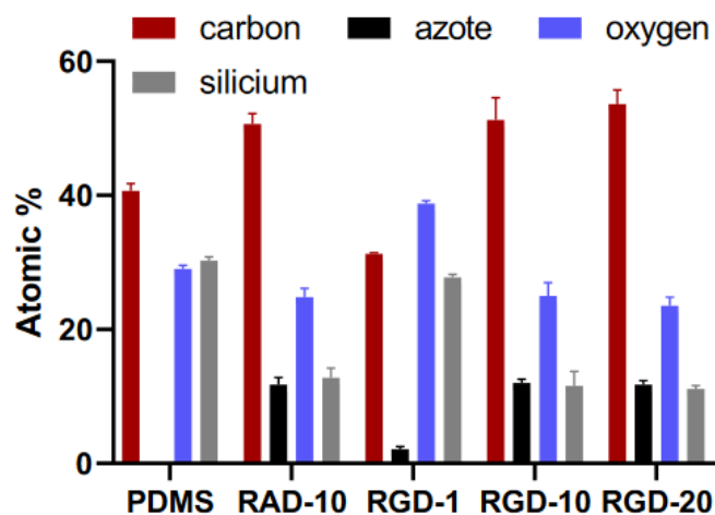
Figure D: Comparative XPS analysis of RGD biofunctionalized PDMS membranes compared to bare PDMS and RAD functionalized membranes. In all five samples, the trio of carbon C1S, silicon S2p, and oxygen O1s characteristic of PDMS is present. Nitrogen N1S is present in all the samples functionalized with peptides. When the concentration exceeds 1 mg/mL, the presence of nitrogen increases, while that of silicon decreases, indicating the formation of a layer.
