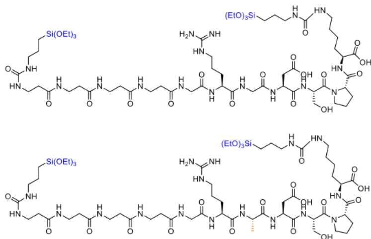
Figure C: Biofunctionalization by peptide-grafting on PDMS. Chemical structures of the hybrid bis-silylated RGD (top) and RAD (bottom) peptides. The triethoxysilane groups (in blue) were introduced at the N-terminus through an ( \beta Ala 4 ) spacer and the side chain of a C-terminal lysine residue, by reaction with isocyanatopropyl triethoxysilane. The difference between the two peptide sequences (methyl side-chain) is highlighted in orange.
