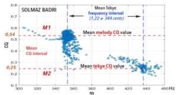
Figure 2: Production of 15 tekye on the same note (F4).
