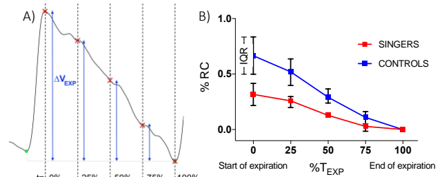
Figure 2: Reduction of the total respiratory volume with time during a singing phrase (A) and percentage of RC contribution to total volume averaged in singers and controls (B).
