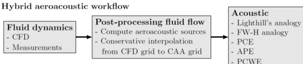
Figure 1: Schematic of the flow diagram of a hybrid aeroacoustic workflow.
