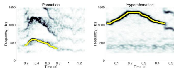
Figure 2: Fundamental frequency estimation for two type of cries: a phonation cry (left) and an hyperphonation cry (right).
