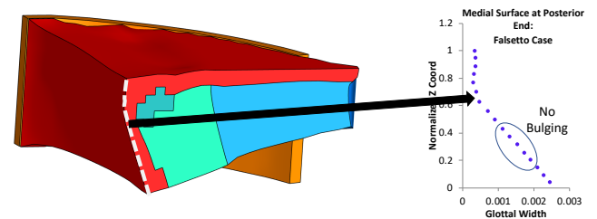
Figure 3: FE Model for falsetto (left) and posterior cross section plot (right) shows no bulging.
