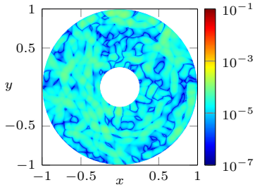
Absolute additive error |u - (u_\theta + p_h^+)|
