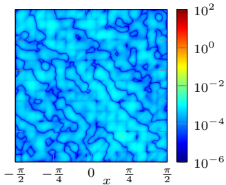
Absolute additive error |u - (u_\theta + p_h^+)|
