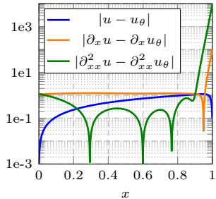
Absolute errors
