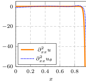
Second-order derivatives
