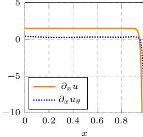
First-order derivatives
