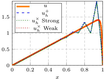
Enriched solutions with \mathbb{P}_1
