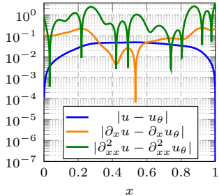
Absolute errors
