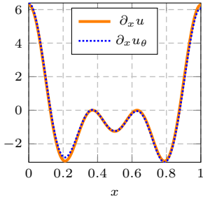
First-order derivatives
