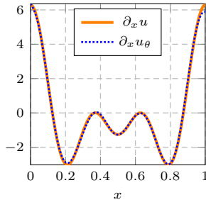
First-order derivatives
