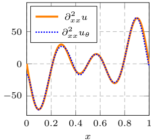
Second-order derivatives
