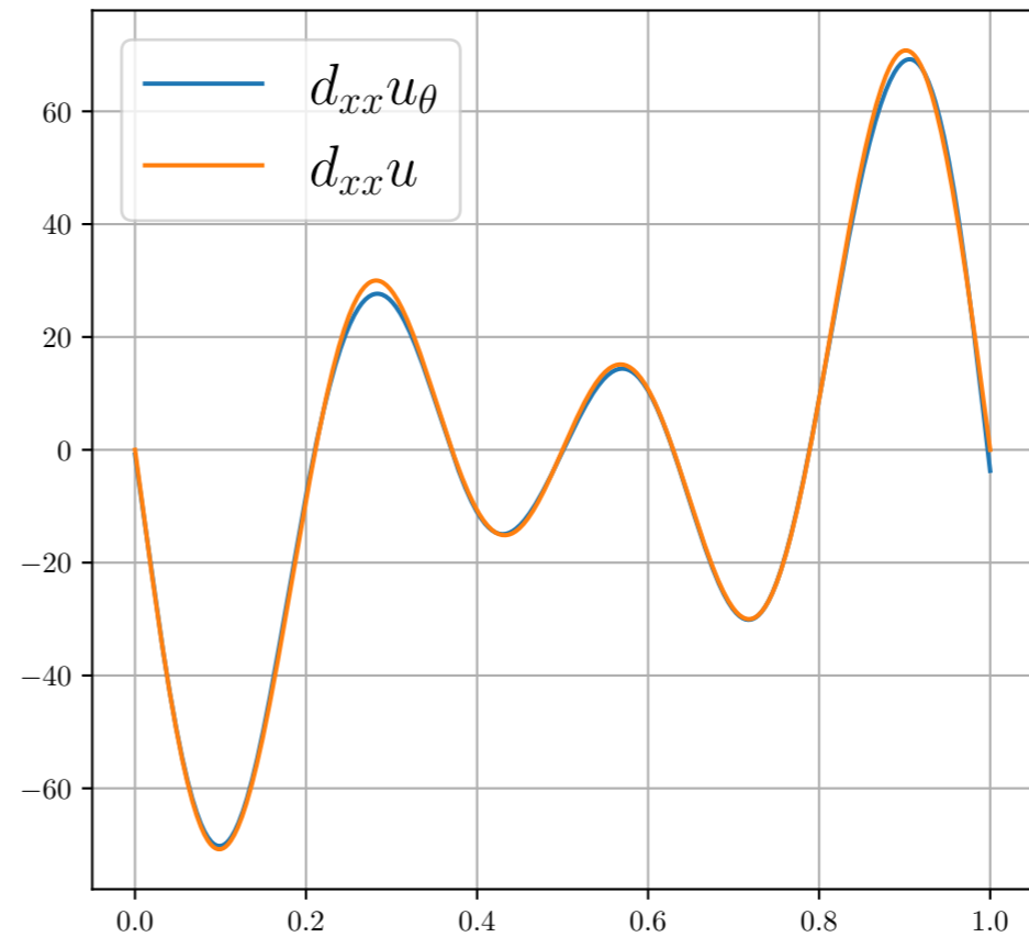
Second-order derivative
