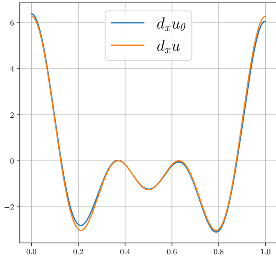
First-order derivative
