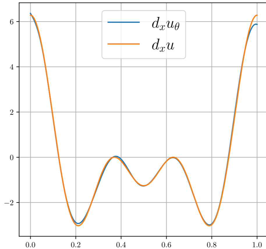
First-order derivative
