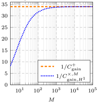
Comparison in H^1 semi-norm
