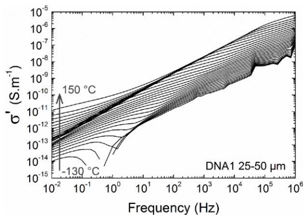
Figure 2 - Isothermal dielectric conductivity of lunar dust simulant against frequency.
