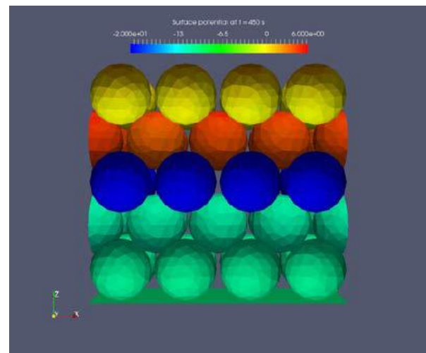
Figure 1 – Simulation of dust layer potential after VUV irradiation inside the DROP lunar dust environment chamber
