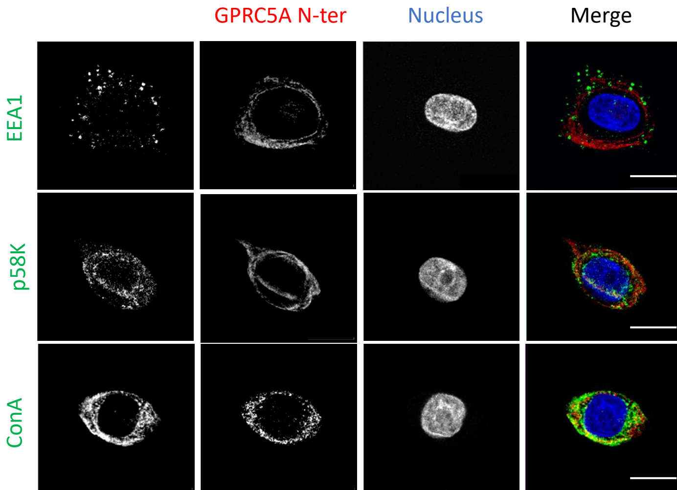
Figure S4: GPRC5A N-terminus immunostaining in red, nucleus counterstaining in blue, the endoplasmic reticulum (Con A), the Golgi apparatus (p58k) or the early endosome vesicles (EEA1) in green. Scale bars: 5 \mu m.
