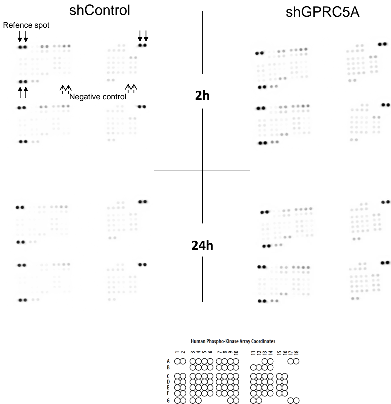
Figure S7: Human phospho-kinase array results and coordinates (by R&D Systems). See legend of the spot position in Table S3 .
