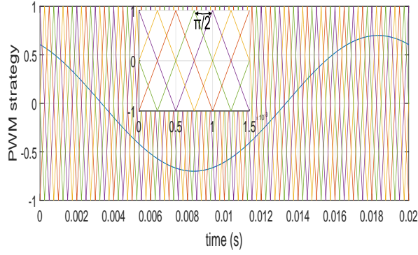
Fig. 7. PWM strategy
