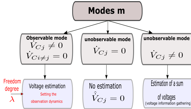
Fig. 9. Observation approach based on mode classification
