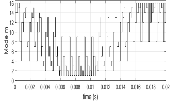
Fig. 8. Switching signal
