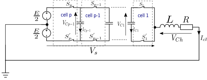
Fig. 1. Multi-cell series inverter.
