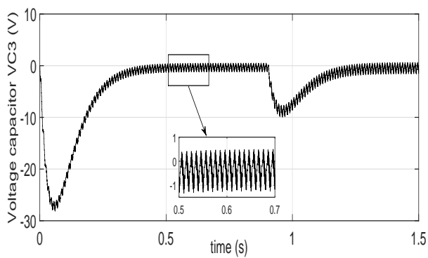
Fig. 15. Observation error of voltage capacitor C3
