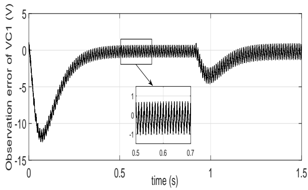
Fig. 13. Observation error of voltage capacitor C1
