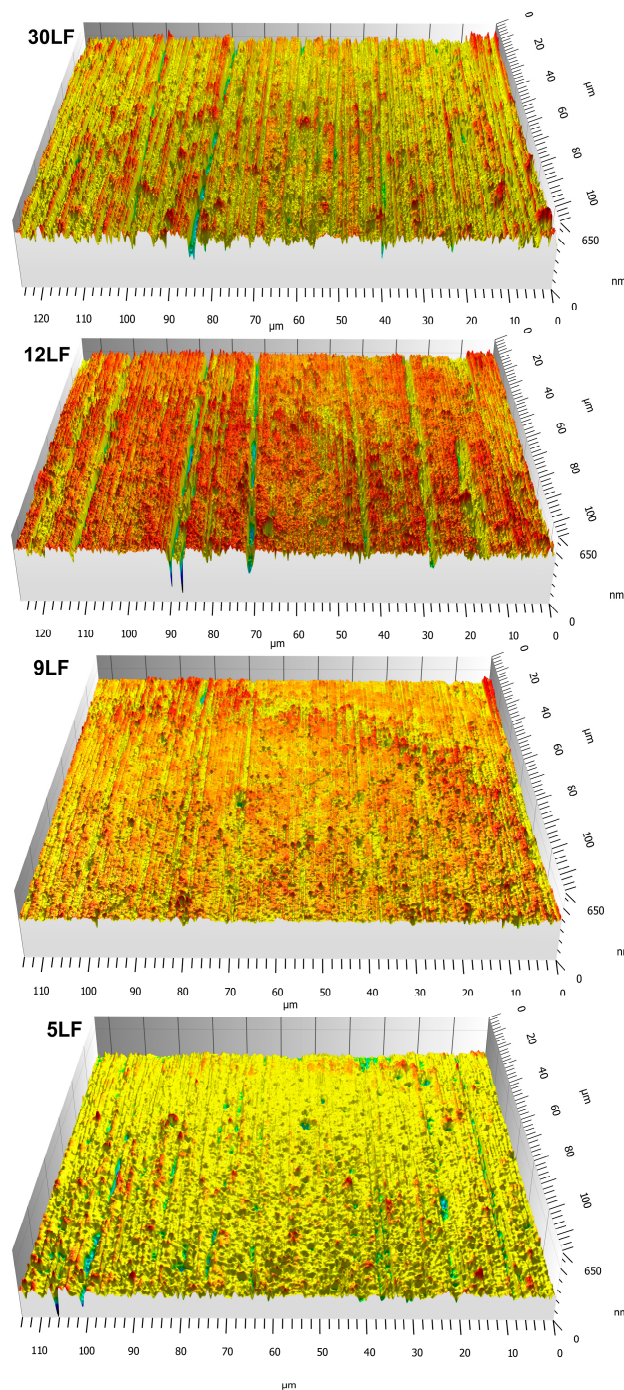
Figure 10. The surfaces of the workpiece after the sequential finishing process using consecutive abrasive films with nominal grain sizes ranging from 30 to 5 \mu\text{m} .
